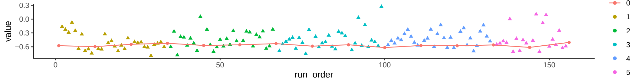
Compound: 1/3-Methylhistidine
