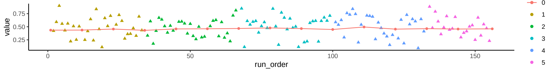
Compound: Trigonelline
