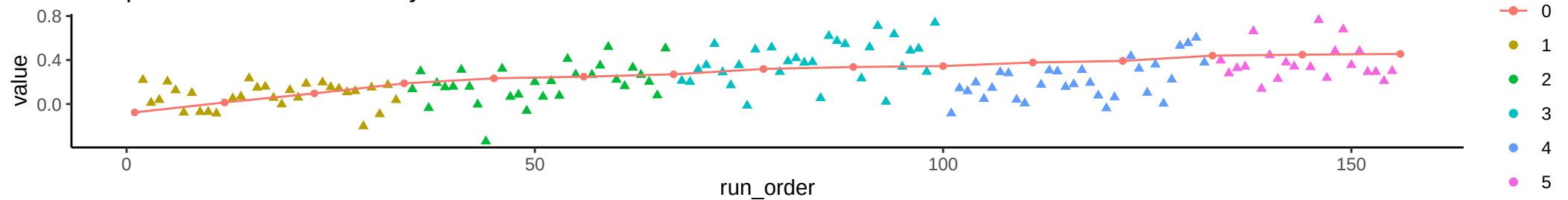
Compound: Inosine
