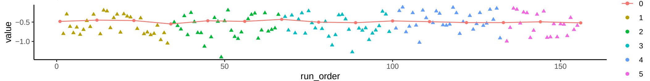
Compound: Uracil
