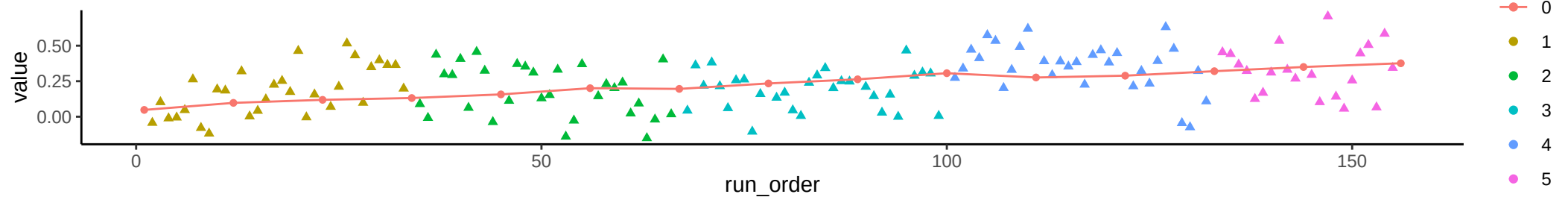
Compound: UDP-Glucose
