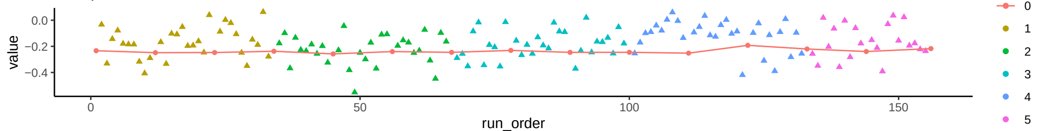
Compound: Lysine
