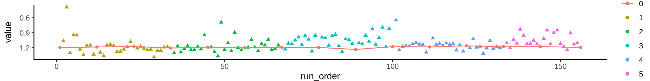
Compound: Ergocalciferol
