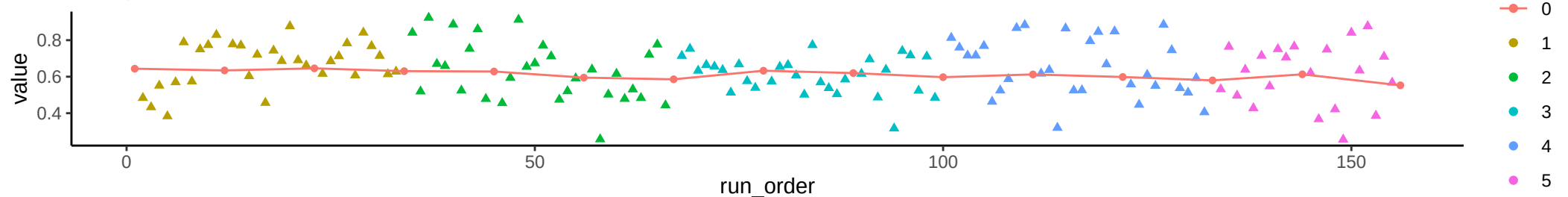
Compound: 2'-Deoxycytidine
