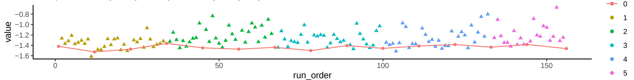
Compound: 2-Hydroxyphenylacetate
