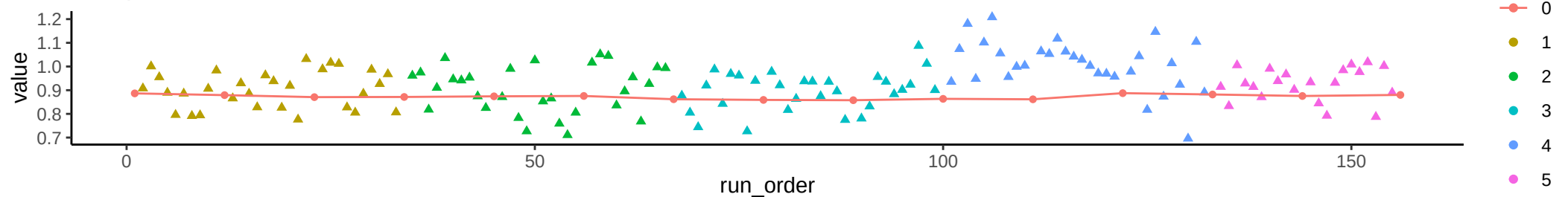
Compound: Urate
