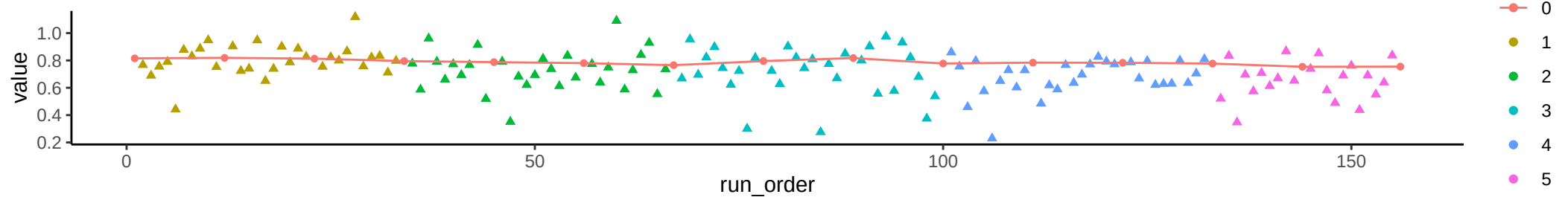
Compound: DHAP/D-GA3P
