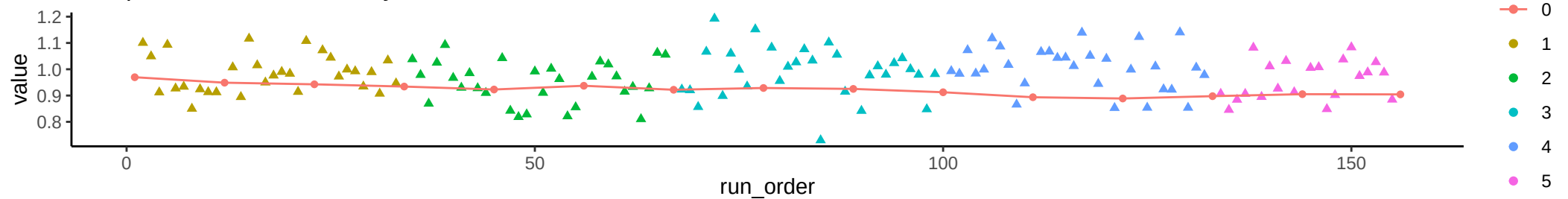
Compound: 2-Hydroxyglutarate
