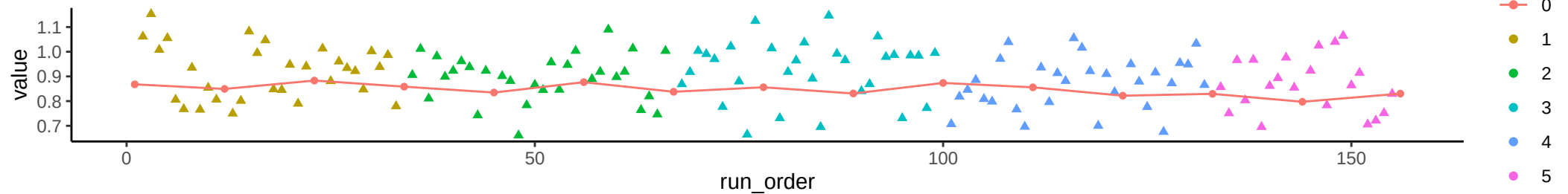
Compound: 1-Methylnicotinamide
