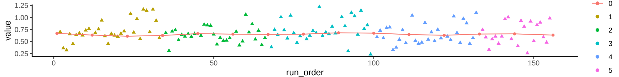
Compound: Dimethylglycine
