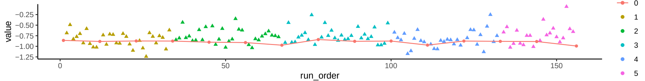
Compound: Tryptophan
