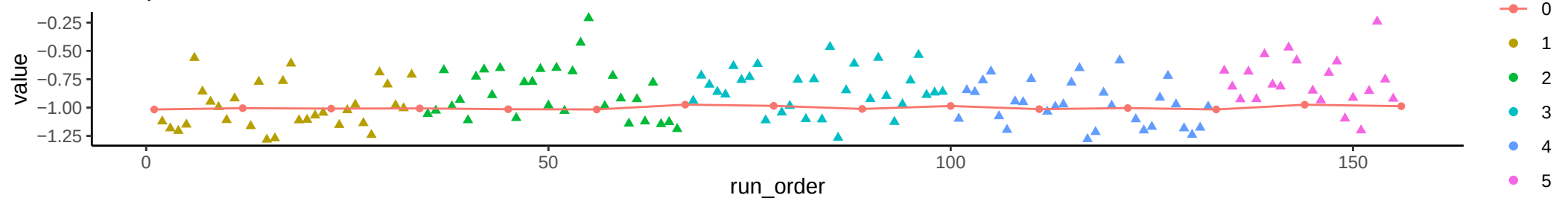
Compound: UMP
