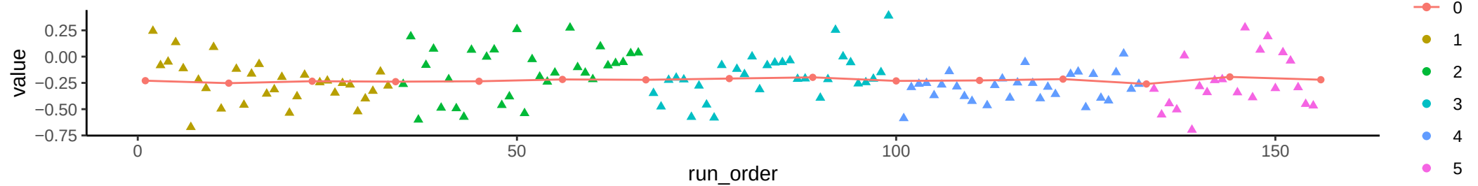
Compound: Tyrosine
