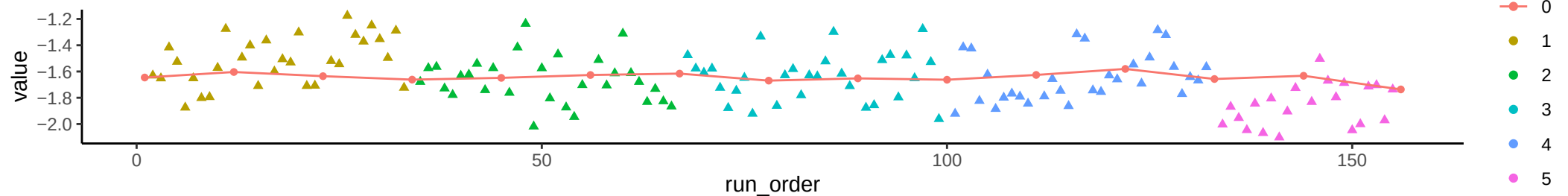
Compound: 2-Aminoadipate
