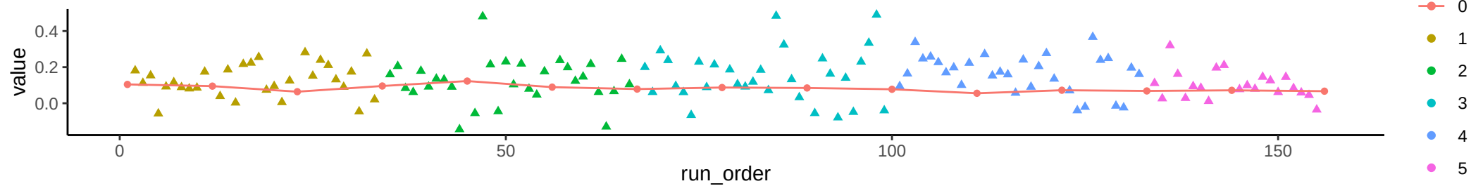
Compound: Tyrosine
