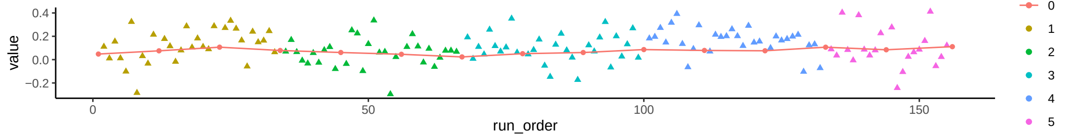
Compound: Threonine
