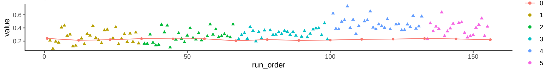
Compound: o-Phosphoethanolamine
