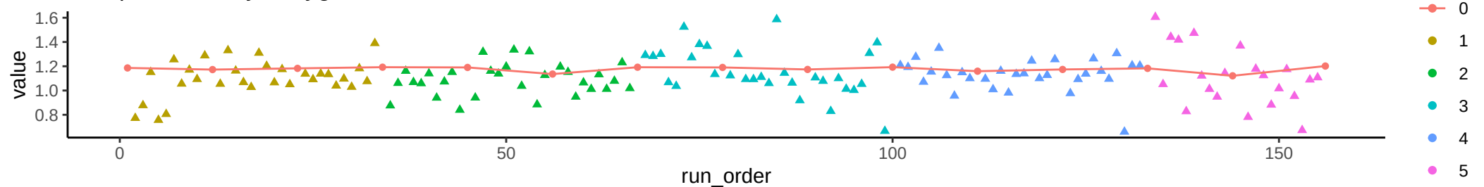
Compound: 2-Hydroxyisobutyrate/2-Hydroxybutyrate
