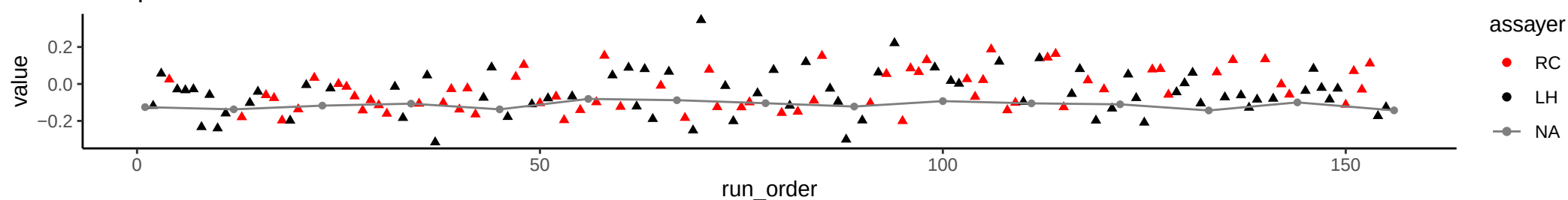
Compound: isoValeric Acid /3-Oxobutanoic Acid/4-Oxobutanoic Acid
