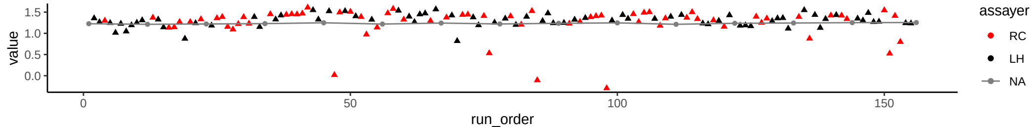
Compound: Anthranilic Acid
