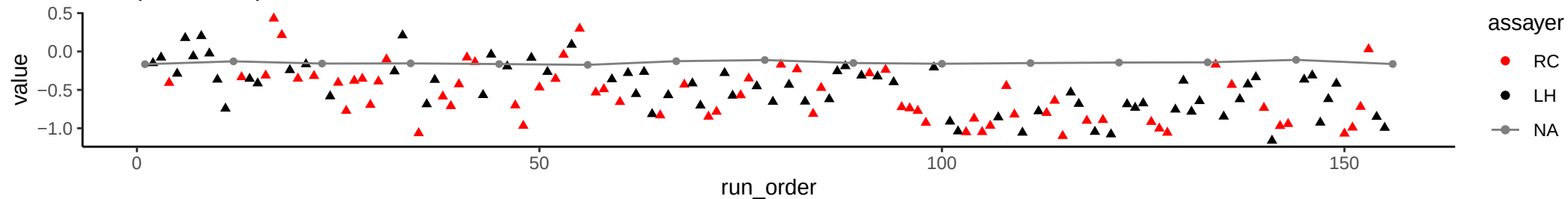
Compound: Azelaic Acid
