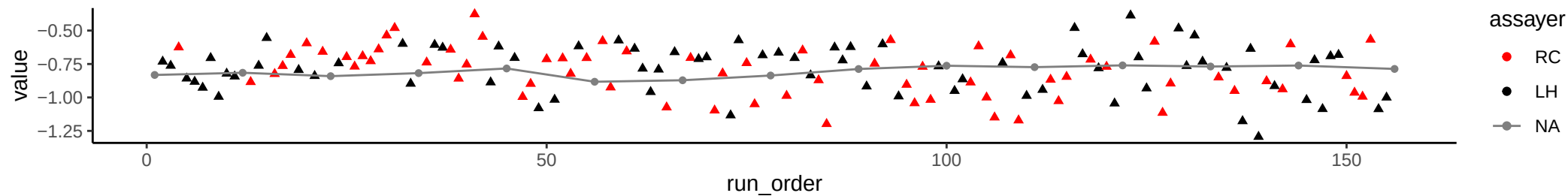
Compound: N-Acetyl-Aspartate (NAA)
