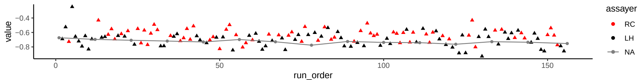
Compound: 3-Methyl-3-Hydroxyglutaric Acid
