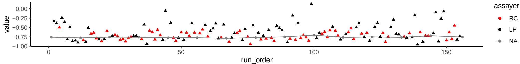
Compound: Oxidized Glutathione
