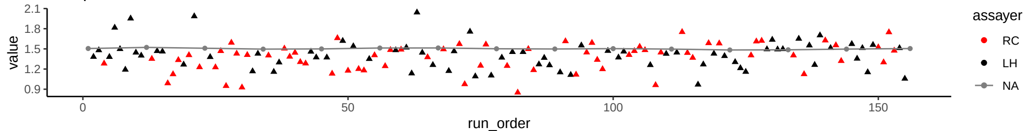
Compound: Glutaric Acid
