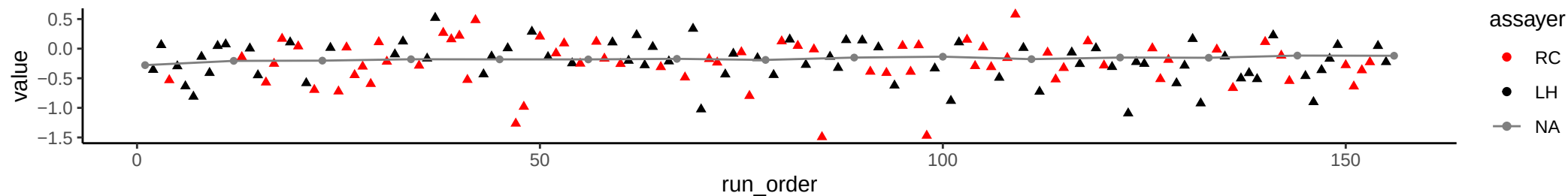
Compound: Palmitic Acid
