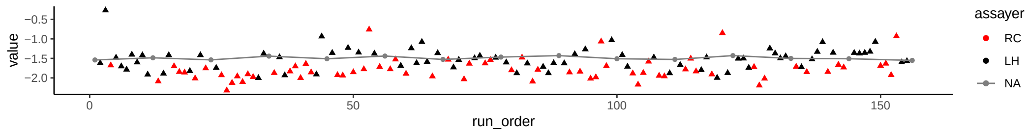
Compound: 2-isoPropylmalic Acid
