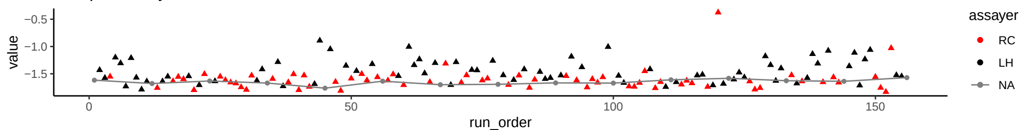
Compound: Hydrocinnamic Acid
