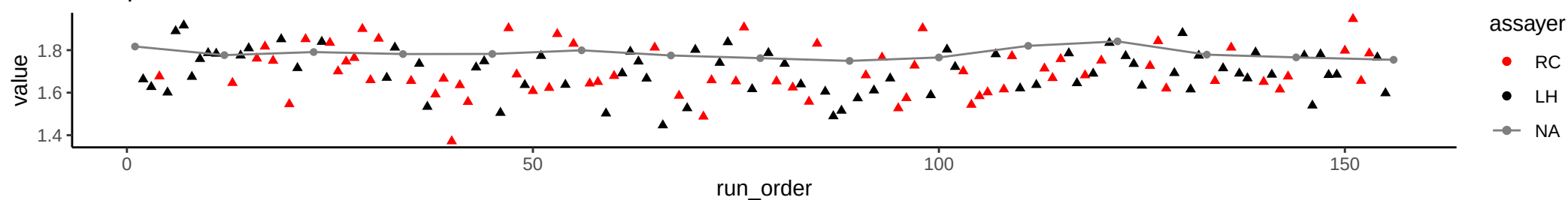
Compound: iso-Leucine /allo-isoLeucine
