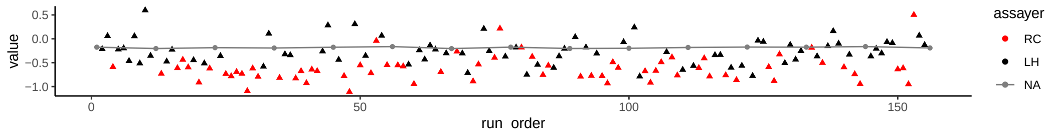
Compound: Adipic Acid / 3-Methylglutaric Acid
