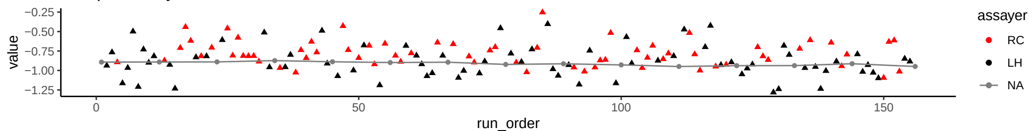
Compound: Cysteinyl-Glycine (Cys-Gly)
