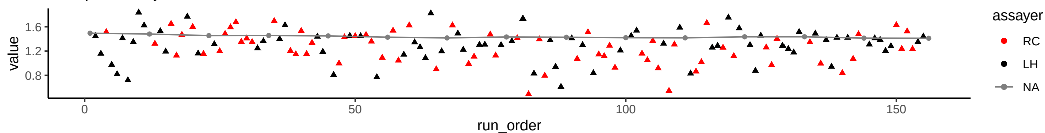
Compound: Kynurenic Acid
