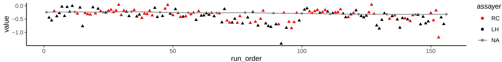
Compound: Myristic Acid
