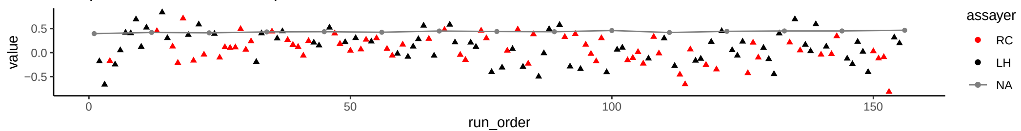
Compound: S-Adenosylmethionine (SAM)
