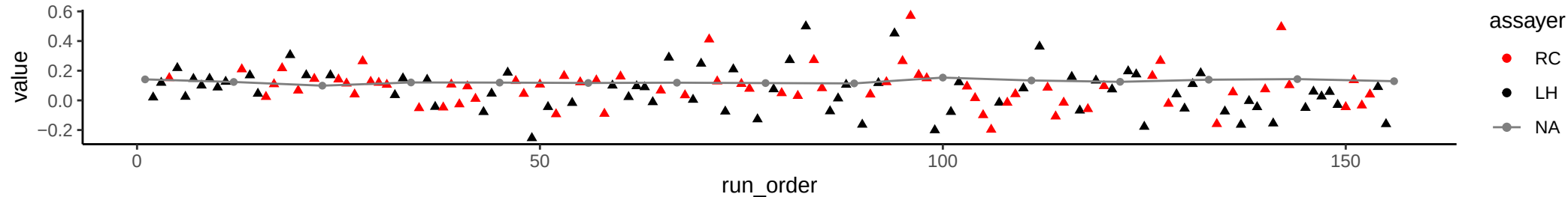
Compound: Xanthurenic Acid
