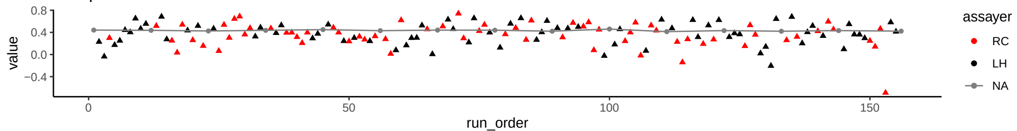
Compound: Ribulose 5-Phosphate
