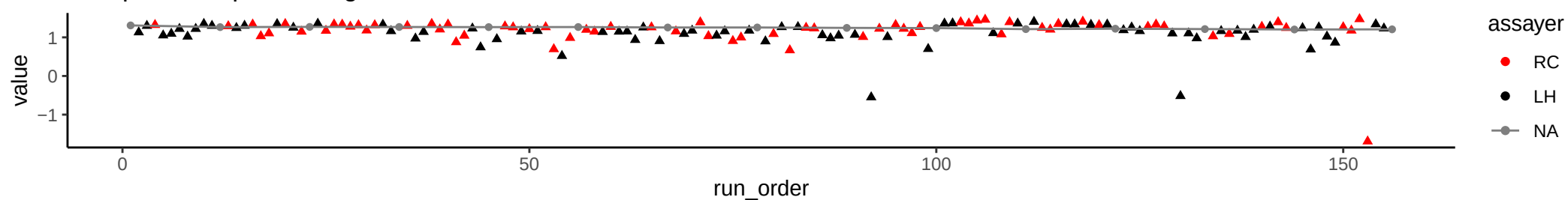
Compound: Alpha-Ketoglutaric Acid
