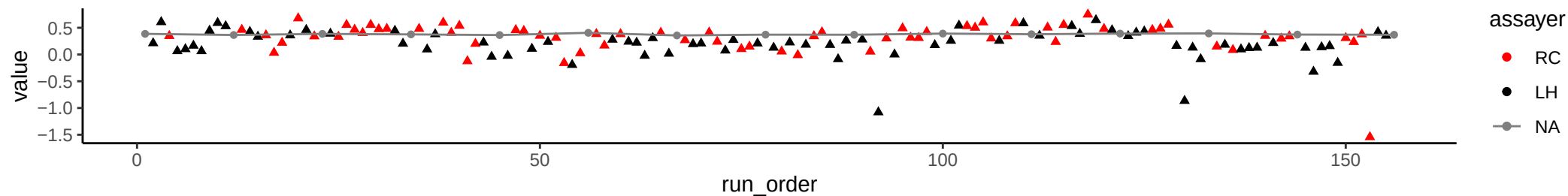
Compound: Reduced Glutathione
