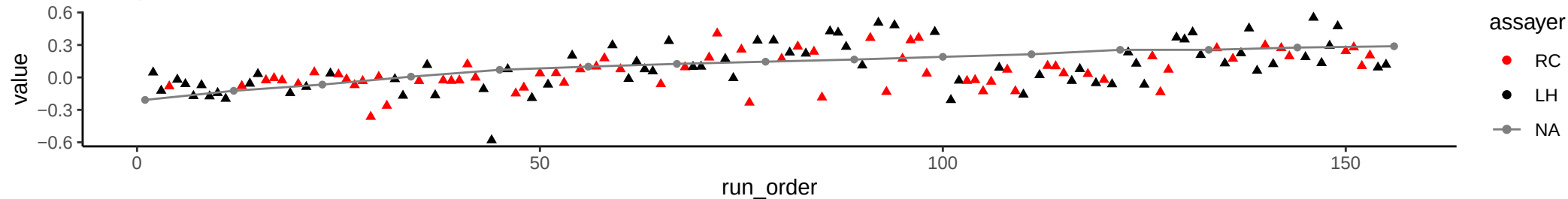
Compound: Indole-2-Carboxylic Acid
