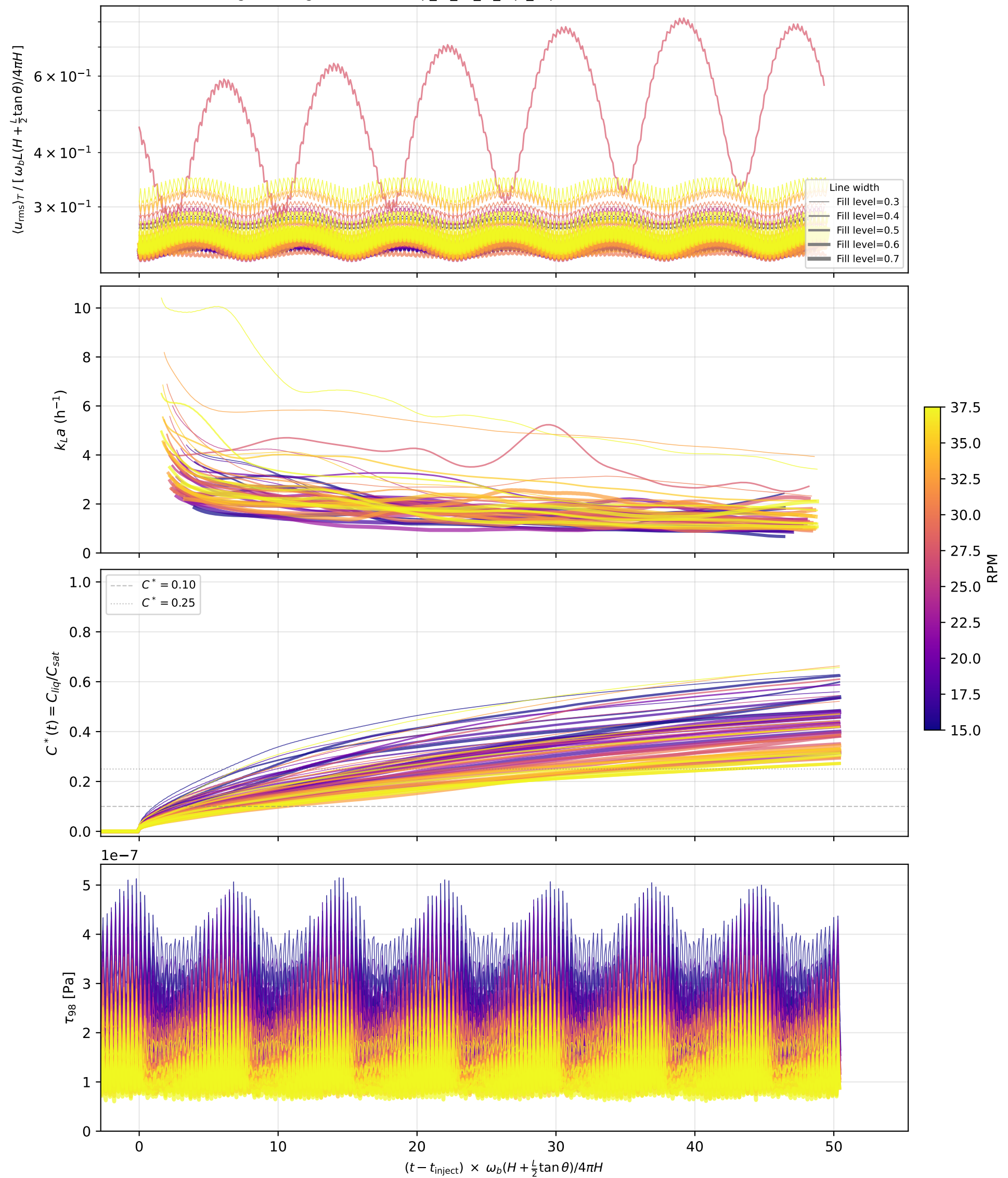
Convergence diagnostics — sweep_fb_fill_l8_mpi_ckpt (50 runs) color=RPM lw=Fill level
