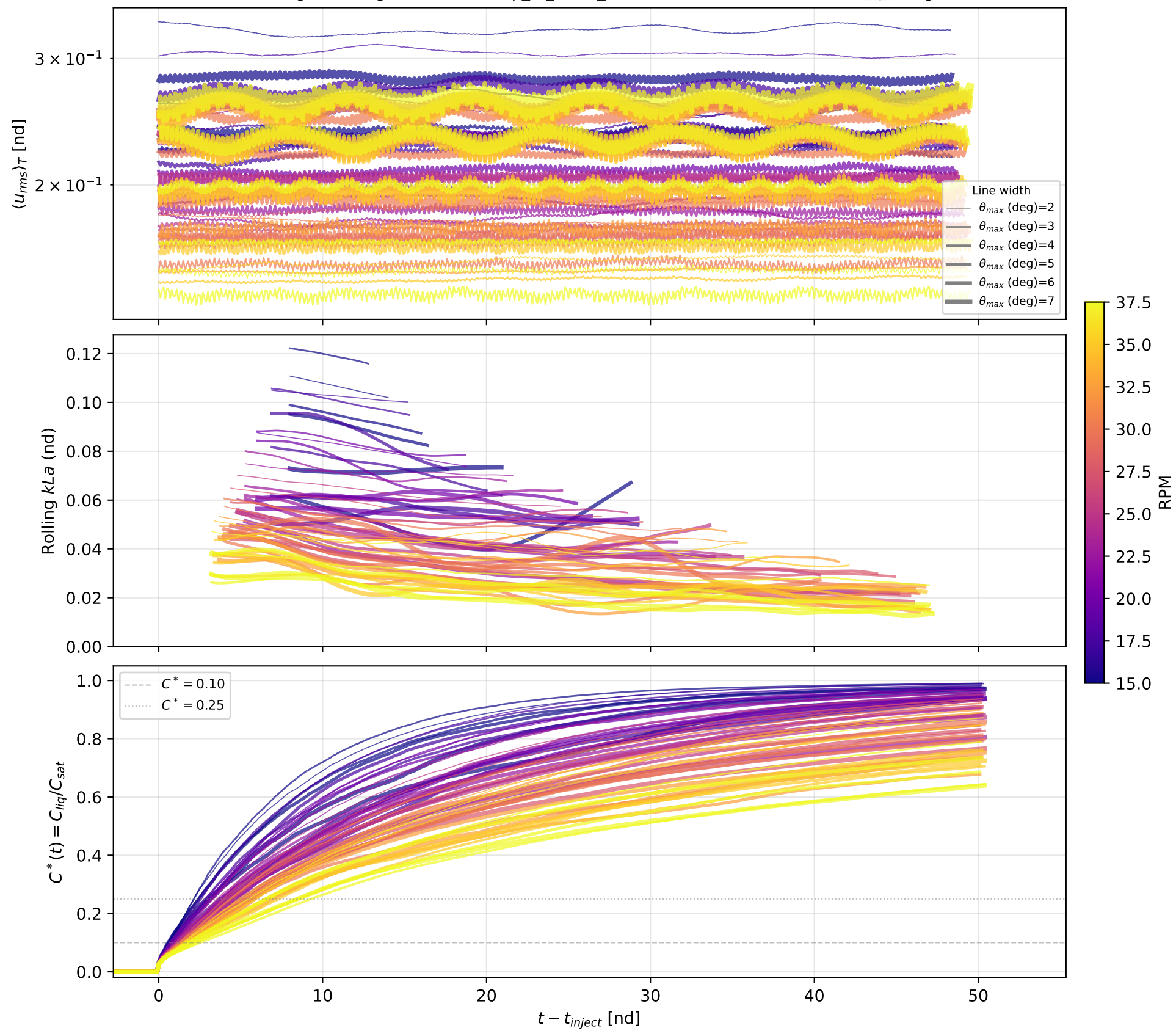
Convergence diagnostics — sweep_fb_theta_l7 (60 runs) color=RPM lw= \theta_{max} (deg)
