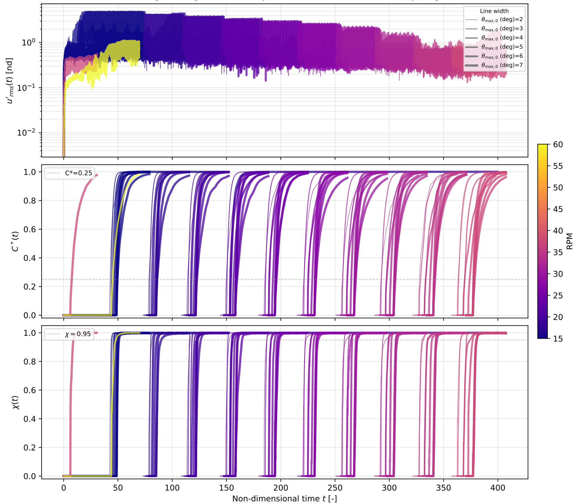
Convergence diagnostics — fidelity 5 (102 runs) color=RPM lw= \theta_{max,0} (deg)
