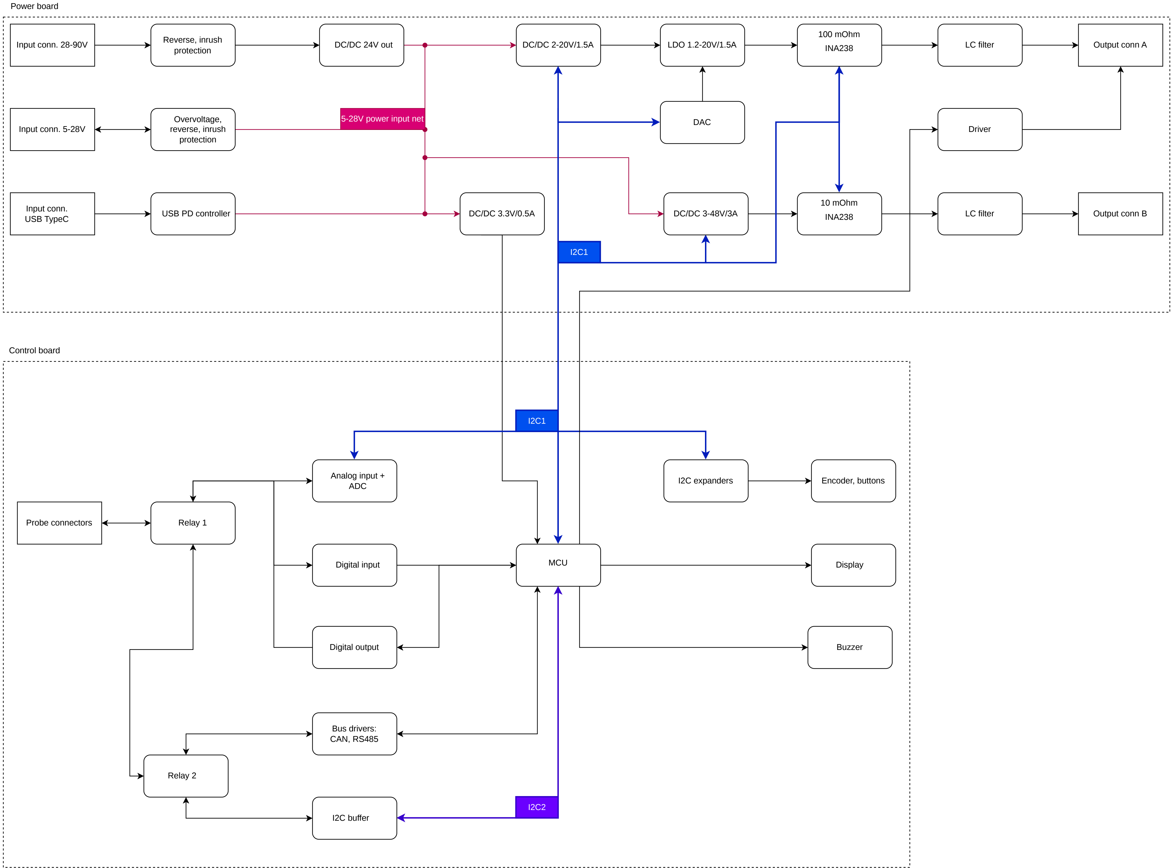
Block diagramm DOGS2 v1
