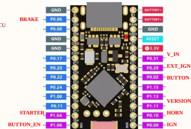
SUPERMINI nrf2840, NICE!NANO
