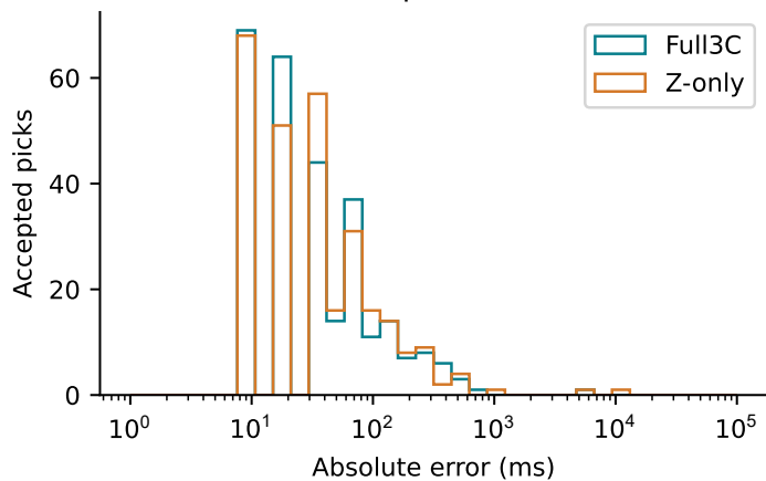
S phase
