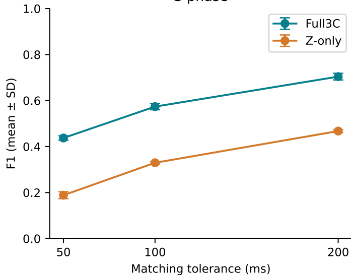
S phase
