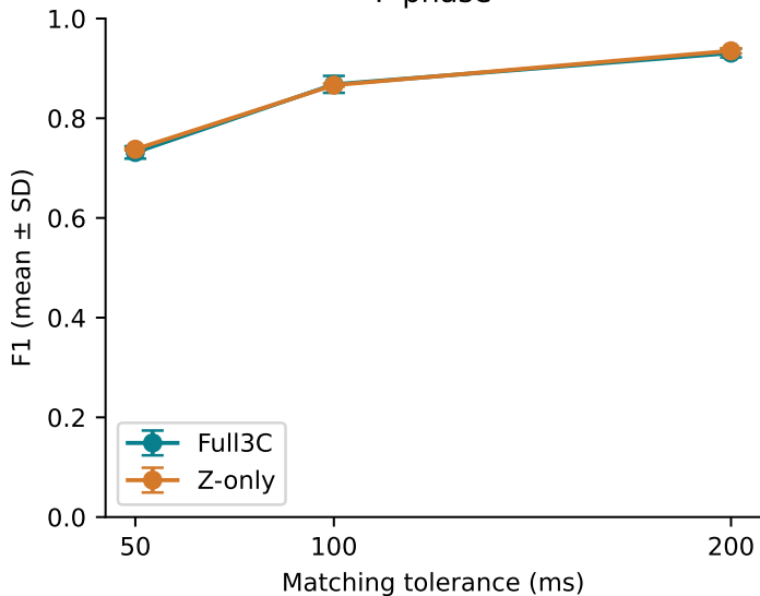
P phase
