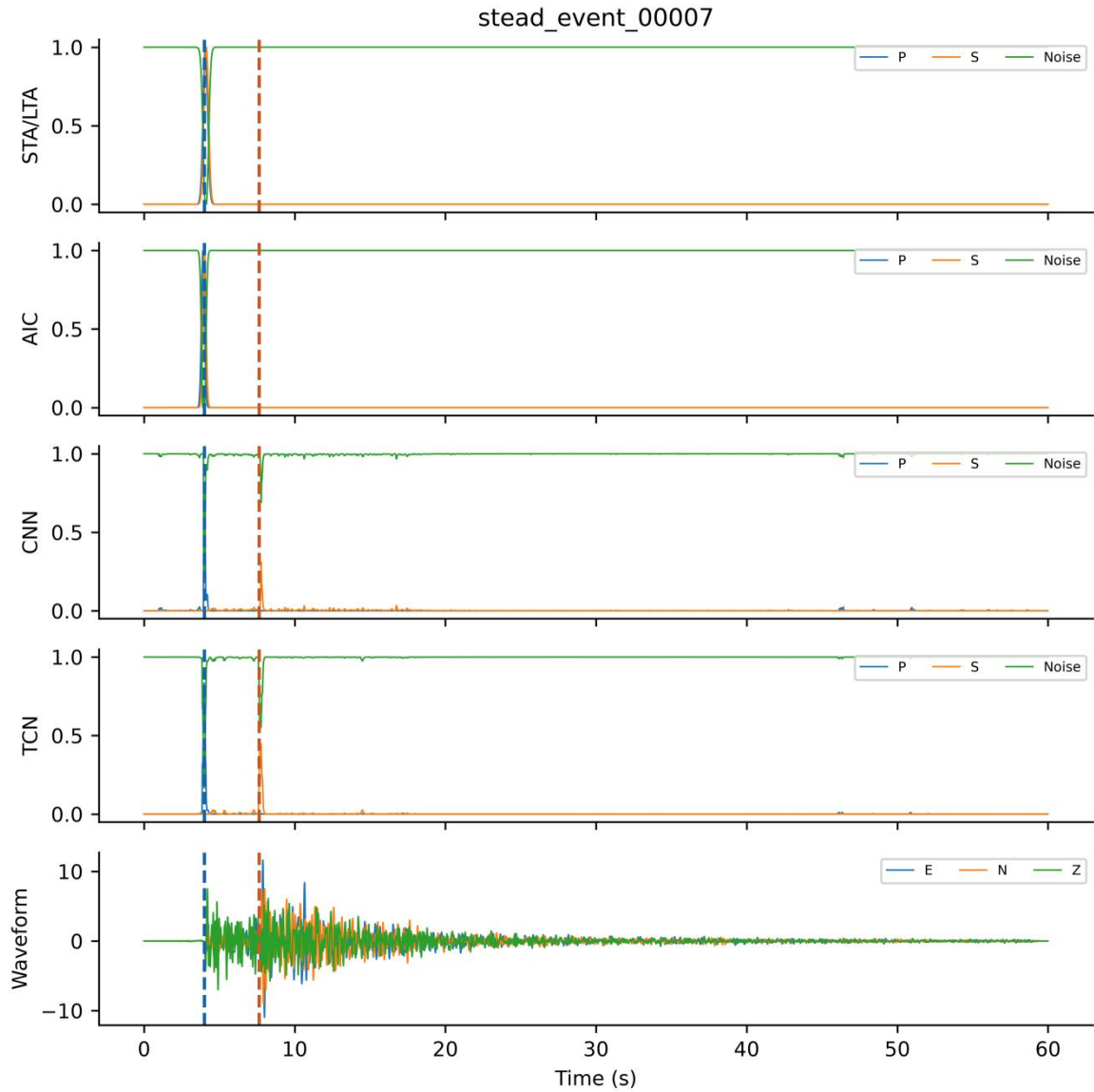
Supplementary Fig. S5. Current final Full3C test tensor for stead_event_00007 . Twelve P/S/noise channels precede conditioned E/N/Z. Dashed lines show true arrivals; Table S1 covers all 330 test tensors.
