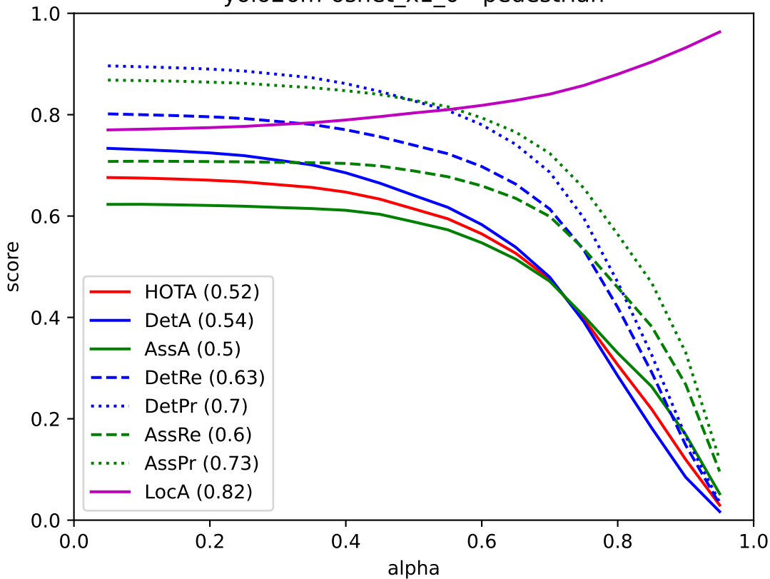
yolo26m-osnet x1 0 - pedestrian
