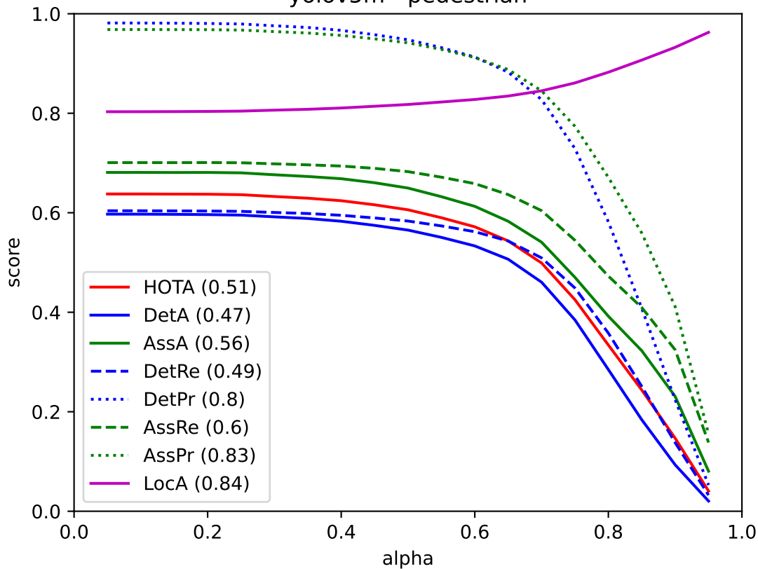
yolov5m - pedestrian
