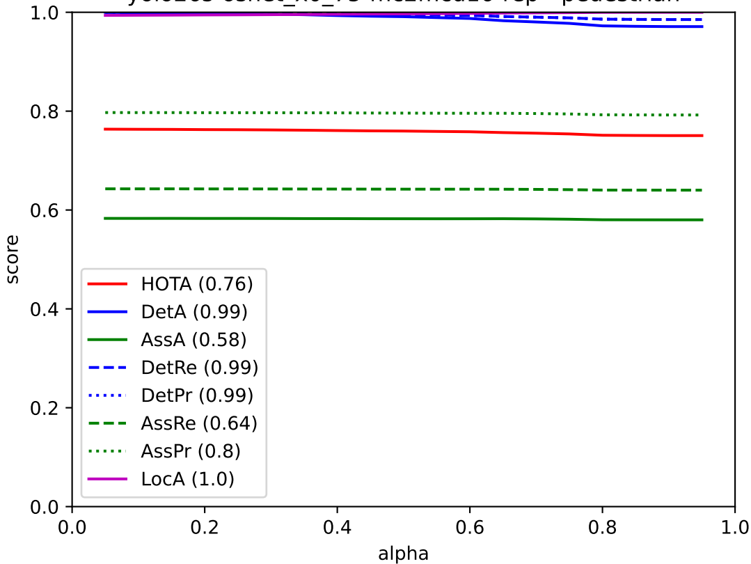
yolo26s-osnet_x0_75-mc2mcd16-rep - pedestrian
