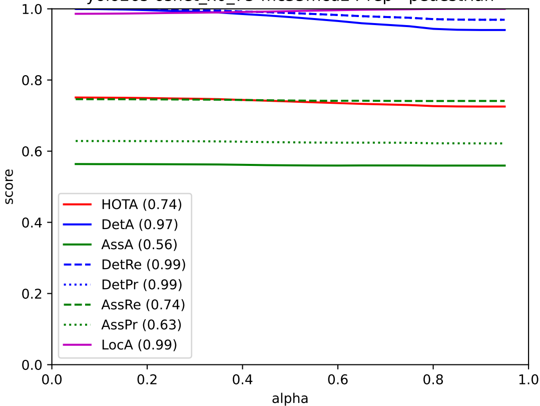
yolo26s-osnet_x0_75-mc35mcd24-rep - pedestrian
