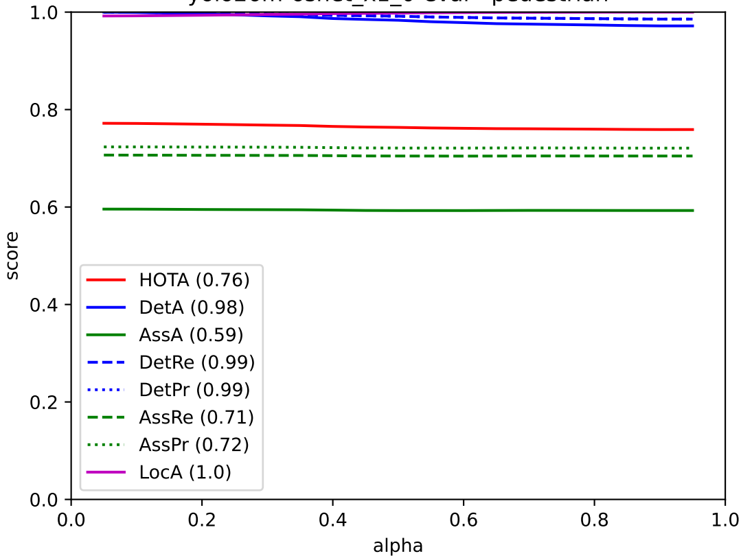
yolo26m-osnet_x1_0-eval - pedestrian
