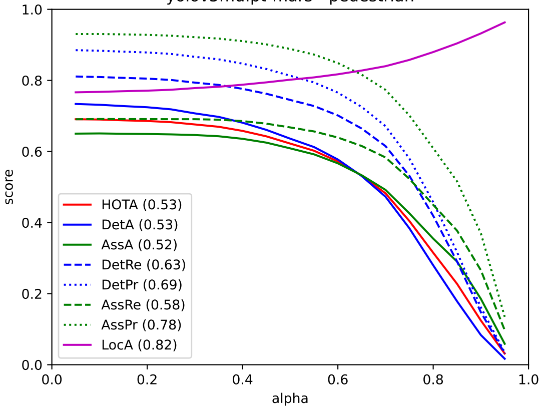
yolov5mu.pt-mars - pedestrian
