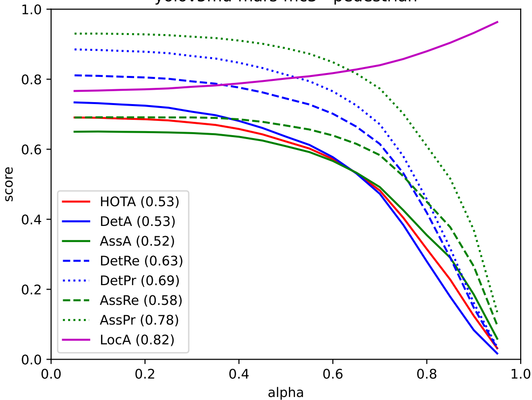
yolov5mu-mars-mc3 - pedestrian
