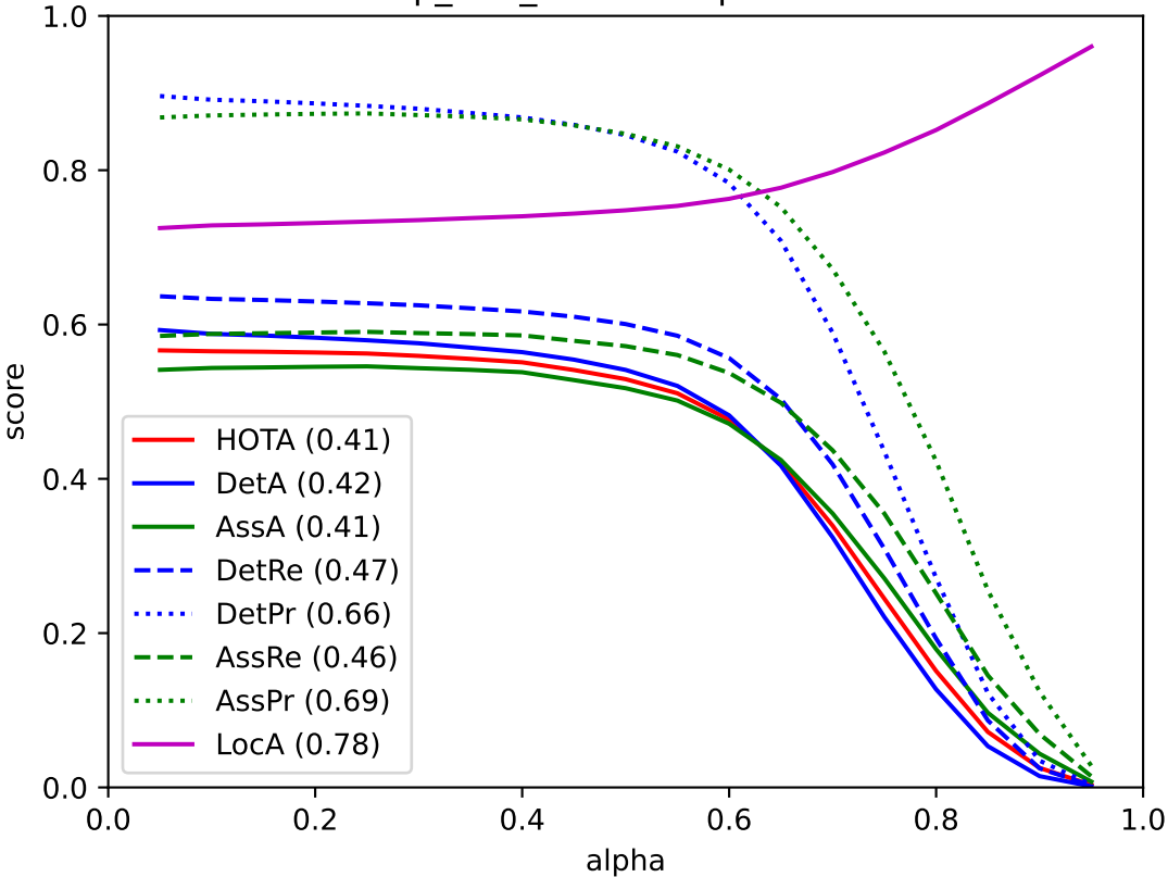
deep sort baseline - pedestrian
