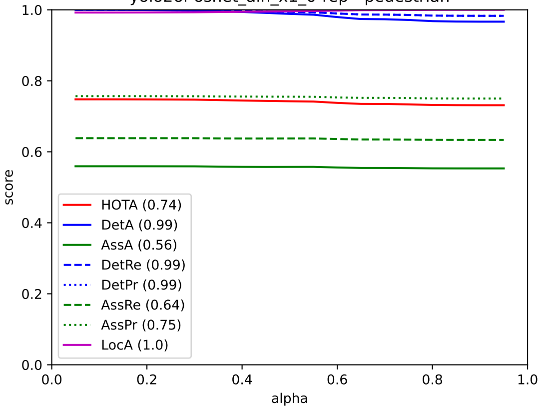
yolo26l-osnet_ain_x1_0-rep - pedestrian
