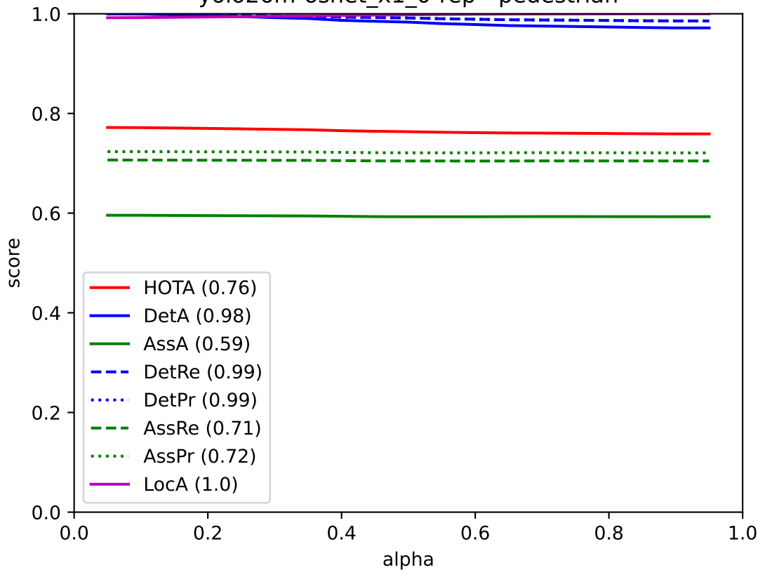
yolo26m-osnet_x1_0-rep - pedestrian
