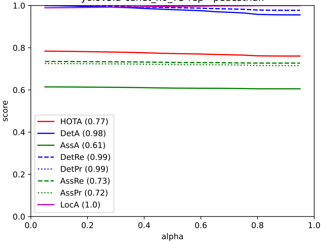
yolov5lu-osnet_x0_75-rep - pedestrian
