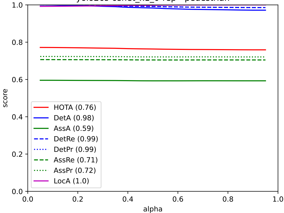
yolo26s-osnet_x1_0-rep - pedestrian
