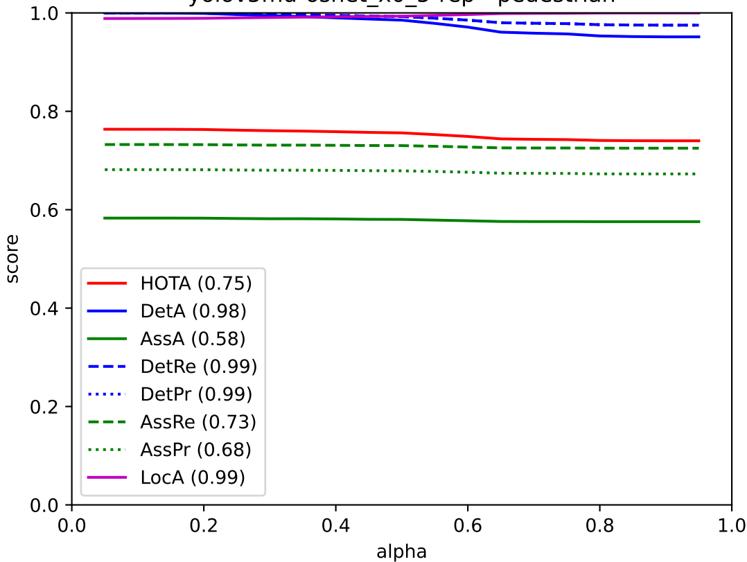
yolov5mu-osnet_x0_5-rep - pedestrian
