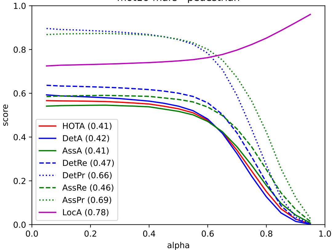
mot16-mars - pedestrian
