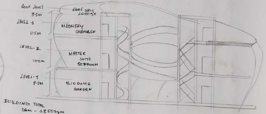
FULL HEIGHT VERTICAL SECTION - Y-Y
