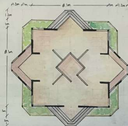
3 LIBRARY FLOOR PLAN
