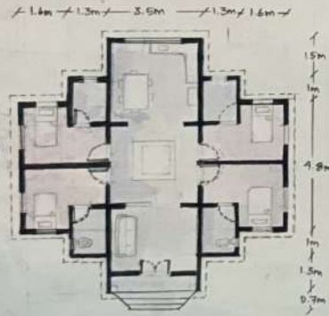
1 SERVANT QUARTERS' GROUND FLOOR PLAN
