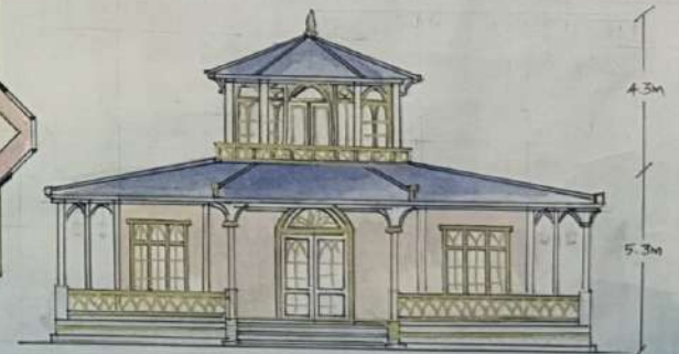
4 GUESTHOUSE FRONT ELEVATION
