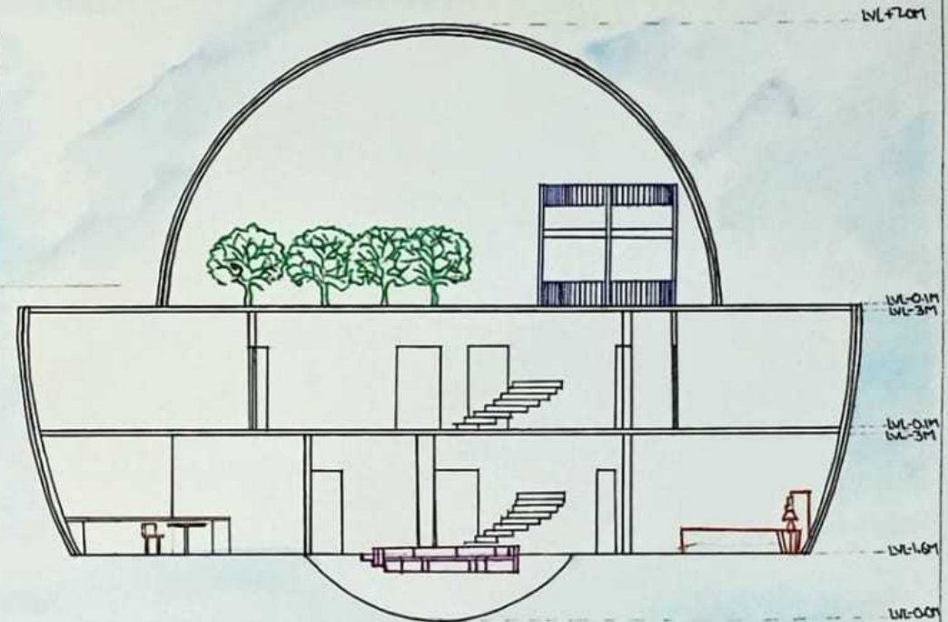
SECTION B-B'
