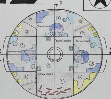
1ST FLOOR PLAN [SCALE-1:100]
