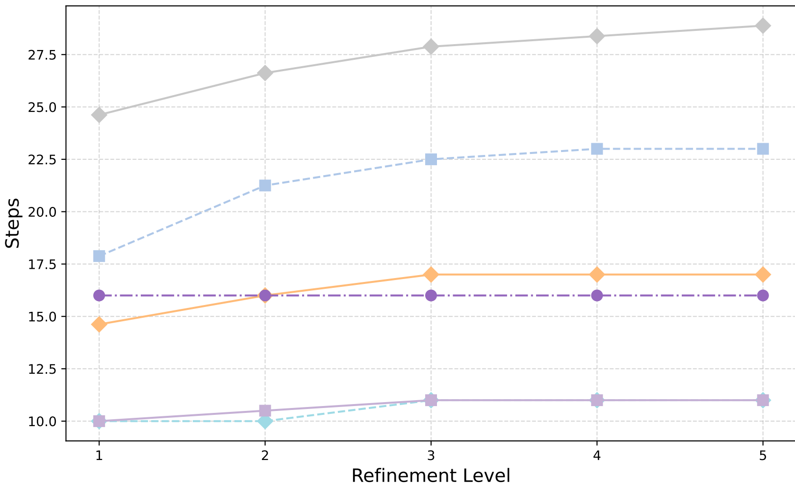
Dirac: V-Cycle (Barycentric) - GMRES Iterations
