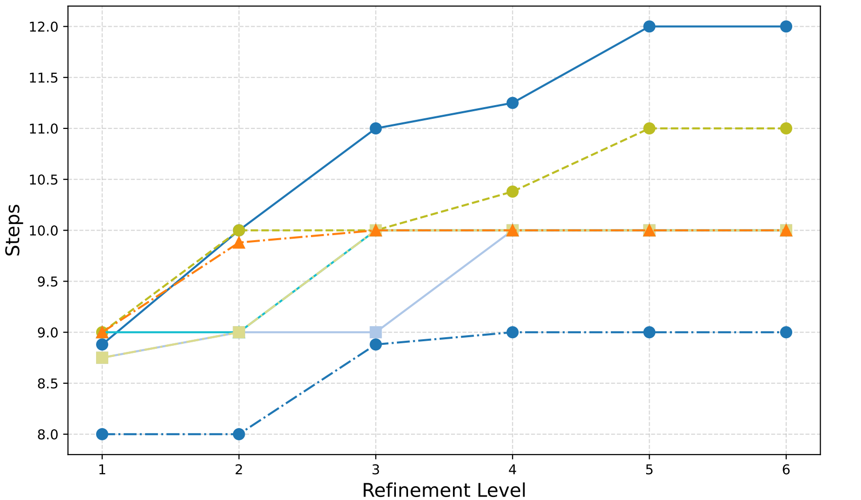
Magnetostatics: V-Cycle (Barycentric) - GMRES Iterations
