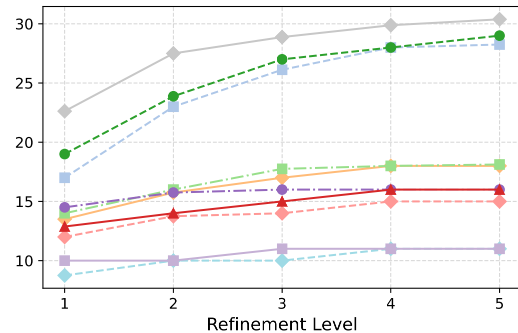
GMRES Iterations
