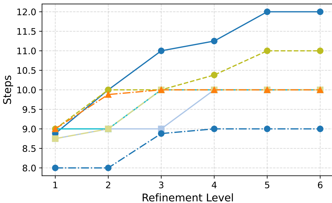
GMRES Iterations
