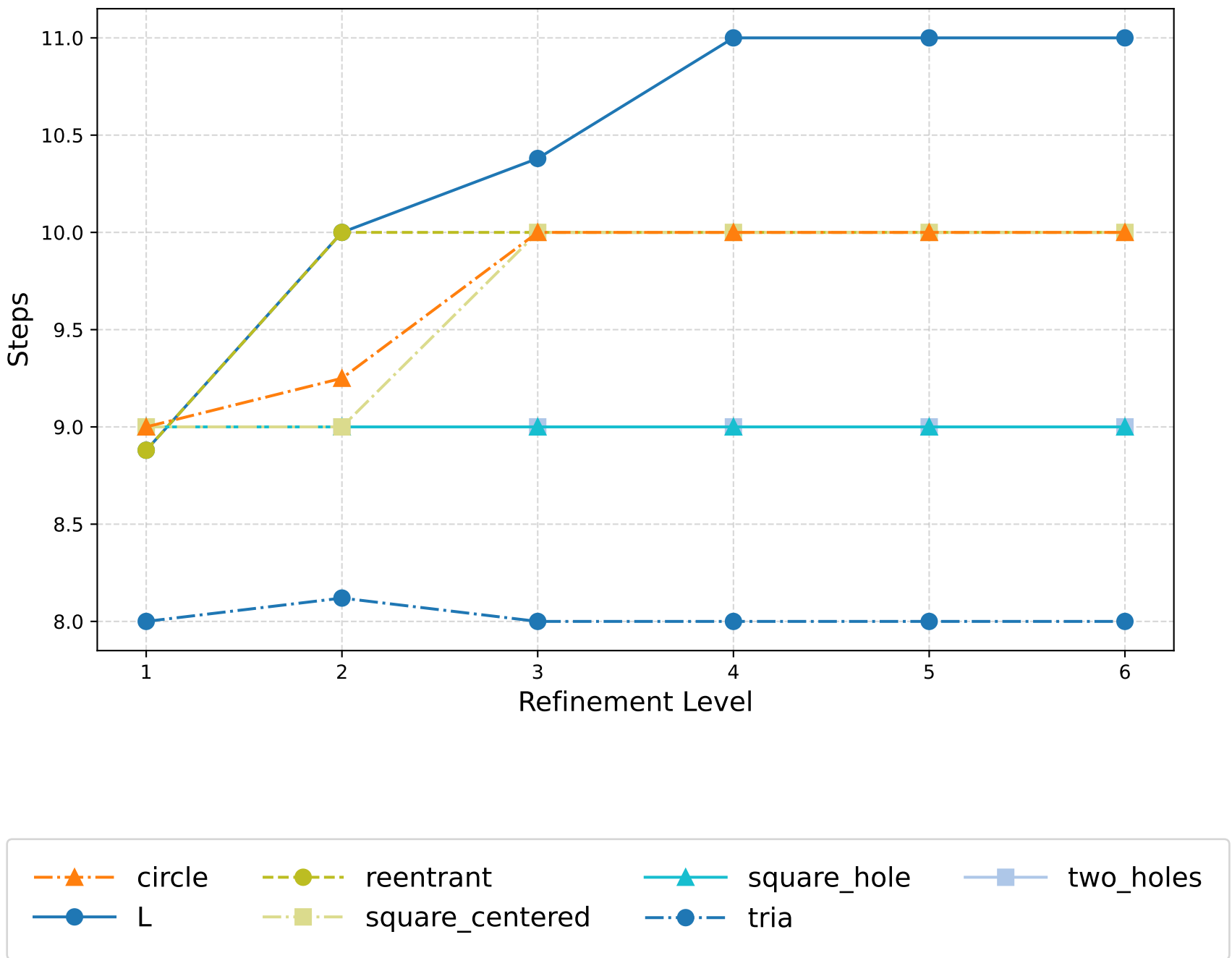
1-form Hodge Laplacian: V-Cycle (Barycentric) - GMRES Iterations
