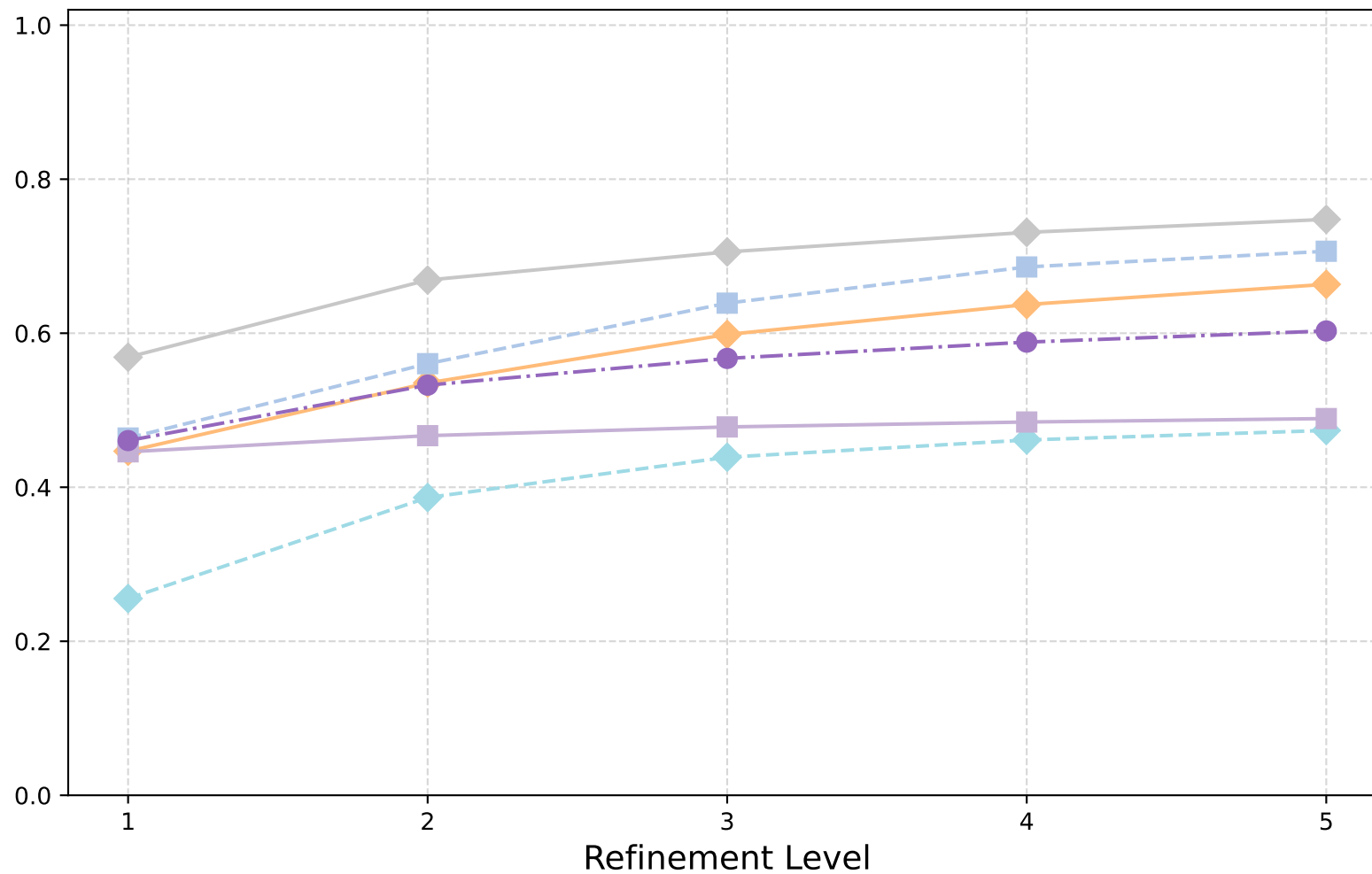
1-form Hodge Laplacian: V-Cycle (Barycentric) - Spectral Radii
