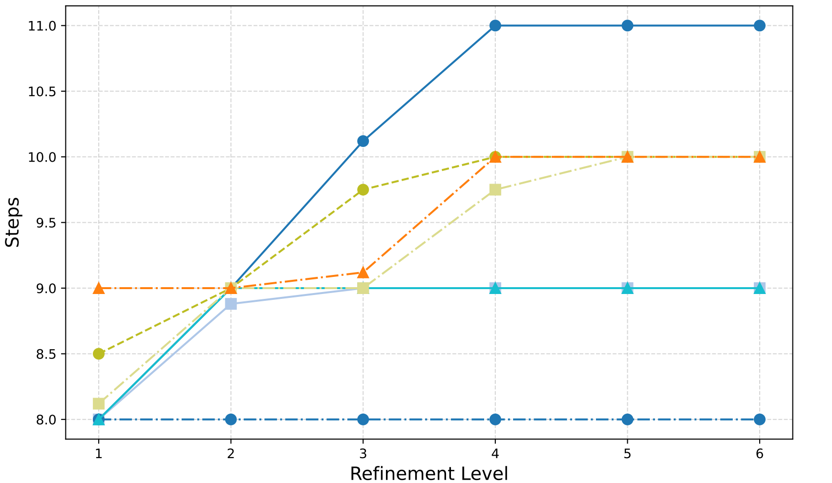
Dirac: W-Cycle (Barycentric) - GMRES Iterations
