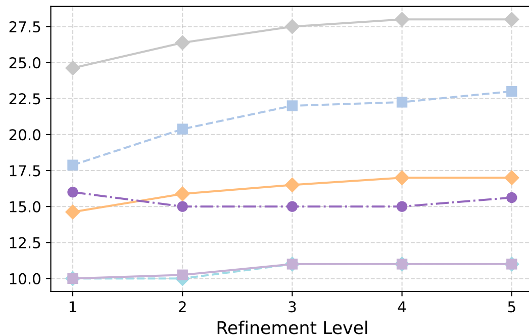
GMRES Iterations
