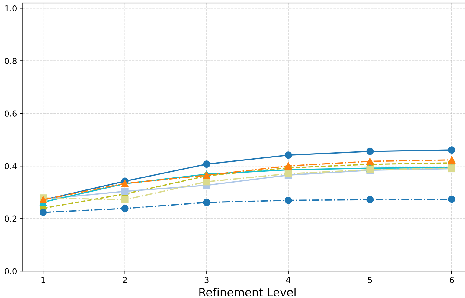
Magnetostatics: W-Cycle (Barycentric) - Spectral Radii
