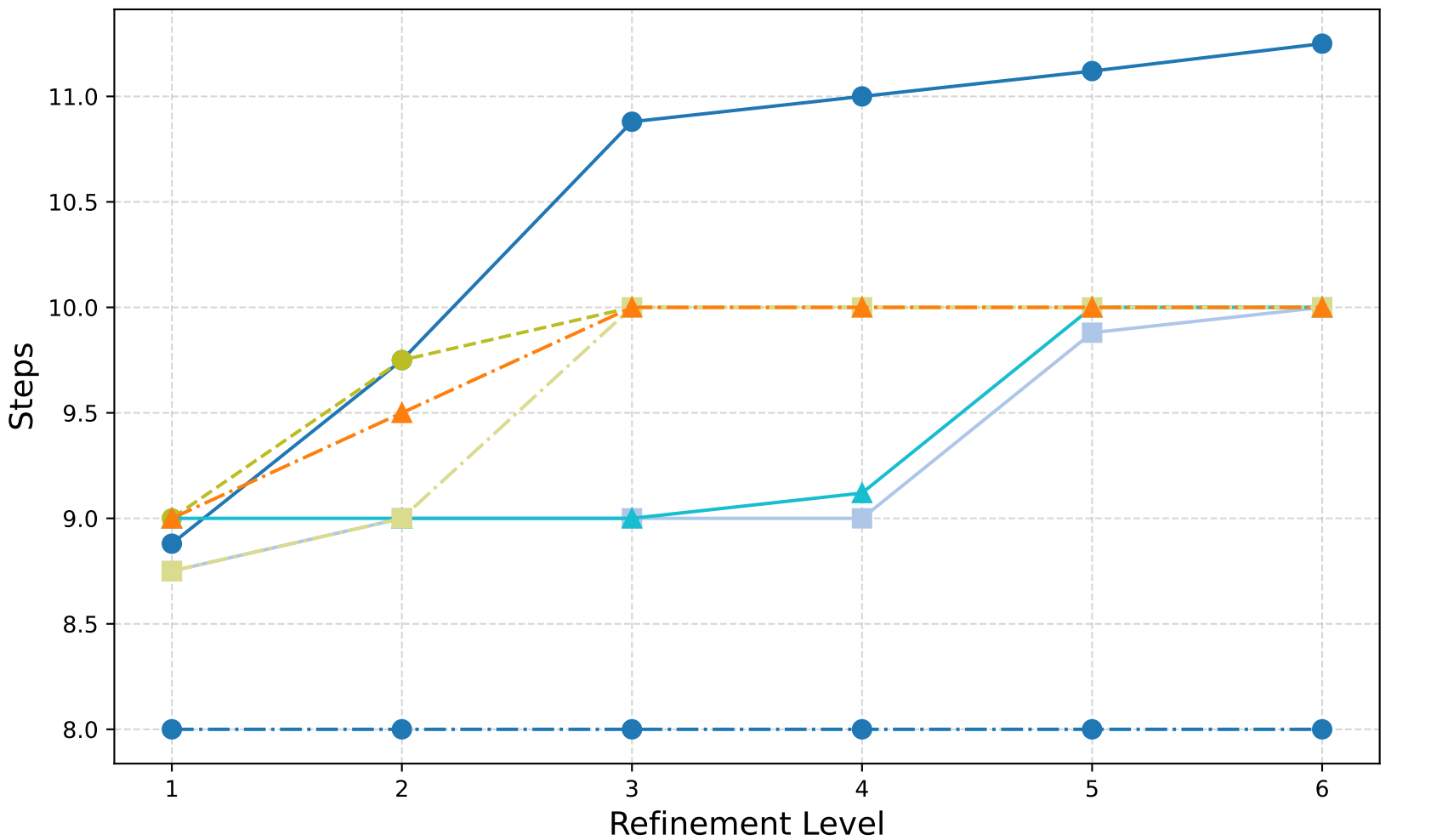
Magnetostatics: W-Cycle (Barycentric) - GMRES Iterations
