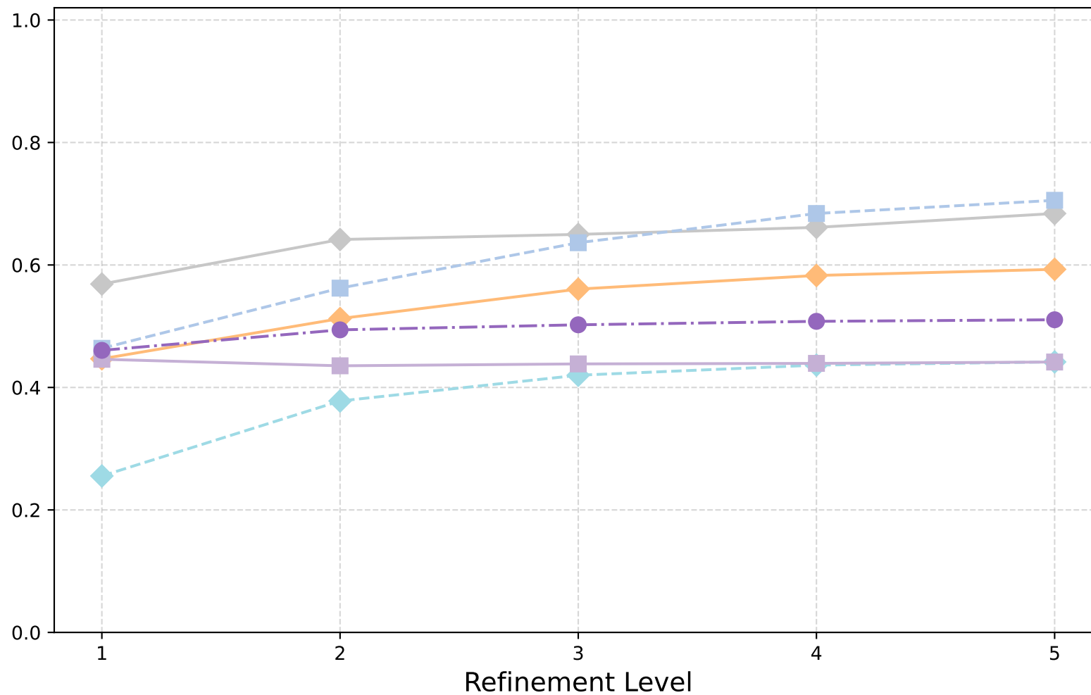
1-form Hodge Laplacian: W-Cycle (Barycentric) - Spectral Radii
