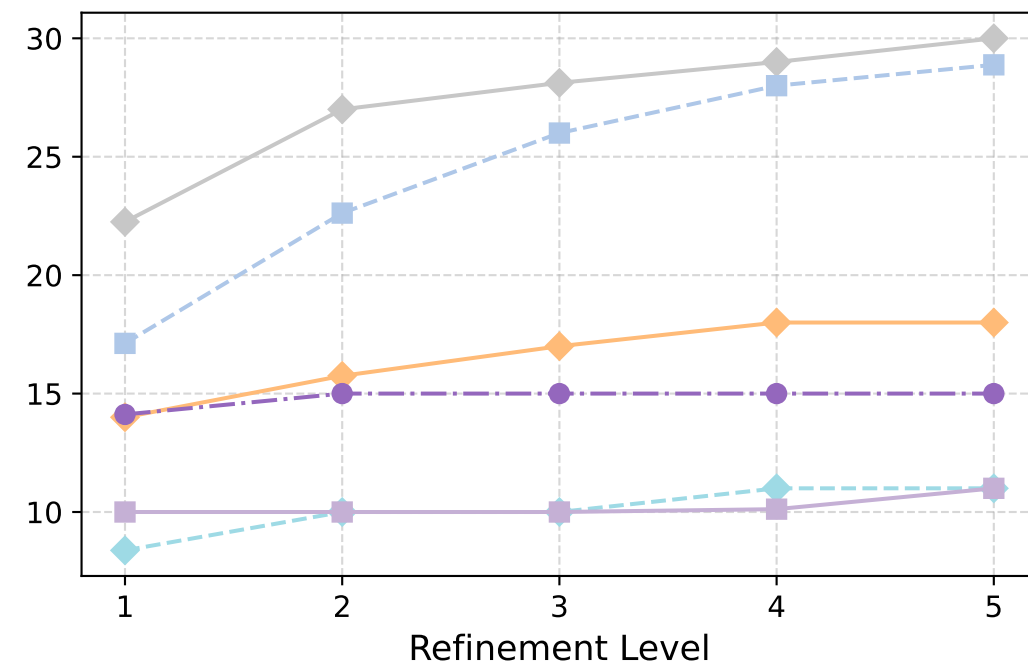
GMRES Iterations
