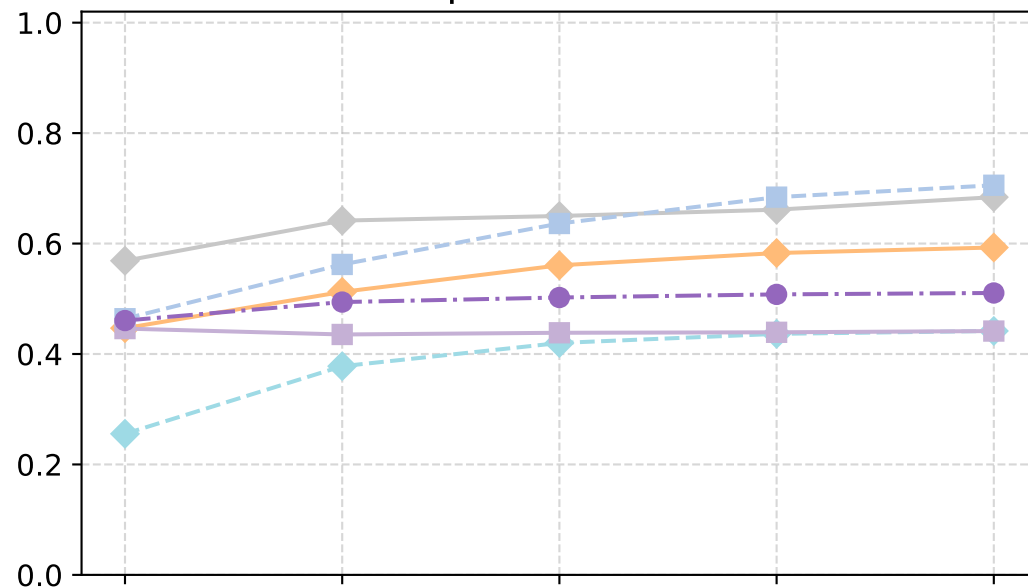
Spectral Radii
