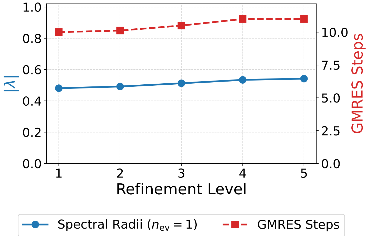
Dirac: V-Cycle (Row Sum)
