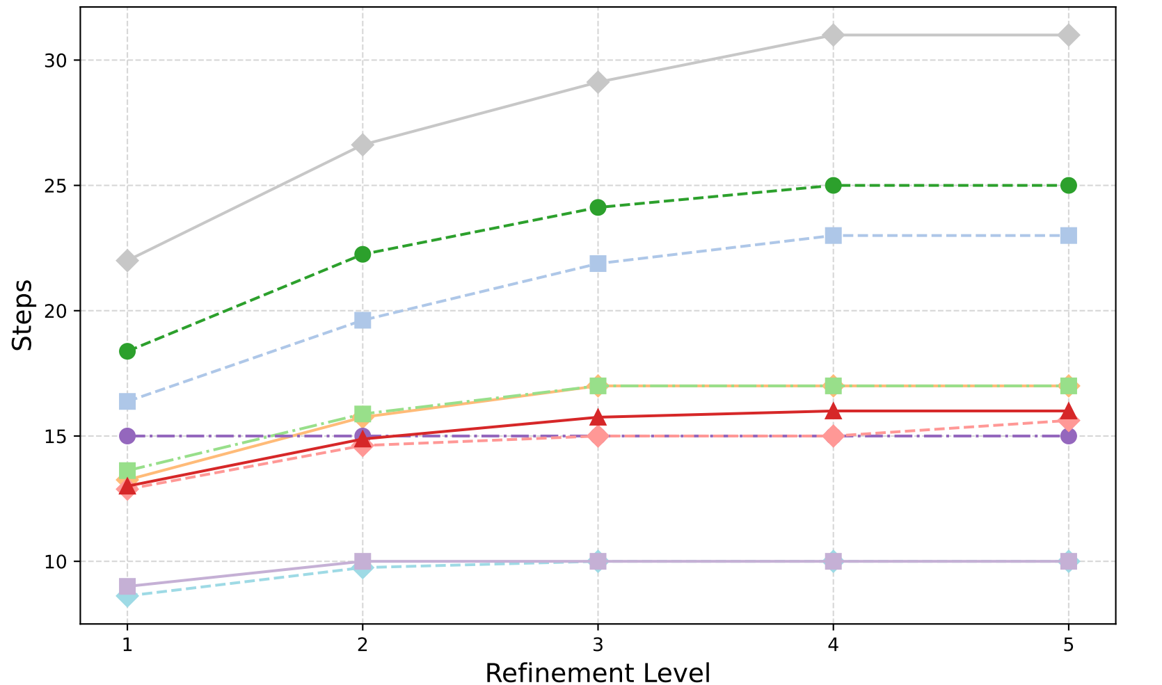
Magnetostatics: V-Cycle (Row Sum) - GMRES Iterations
