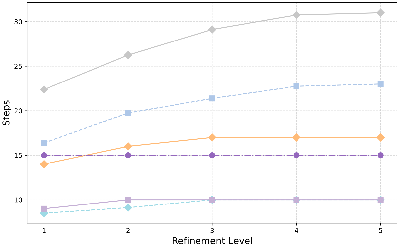
1-form Hodge Laplacian: V-Cycle (Row Sum) - GMRES Iterations
