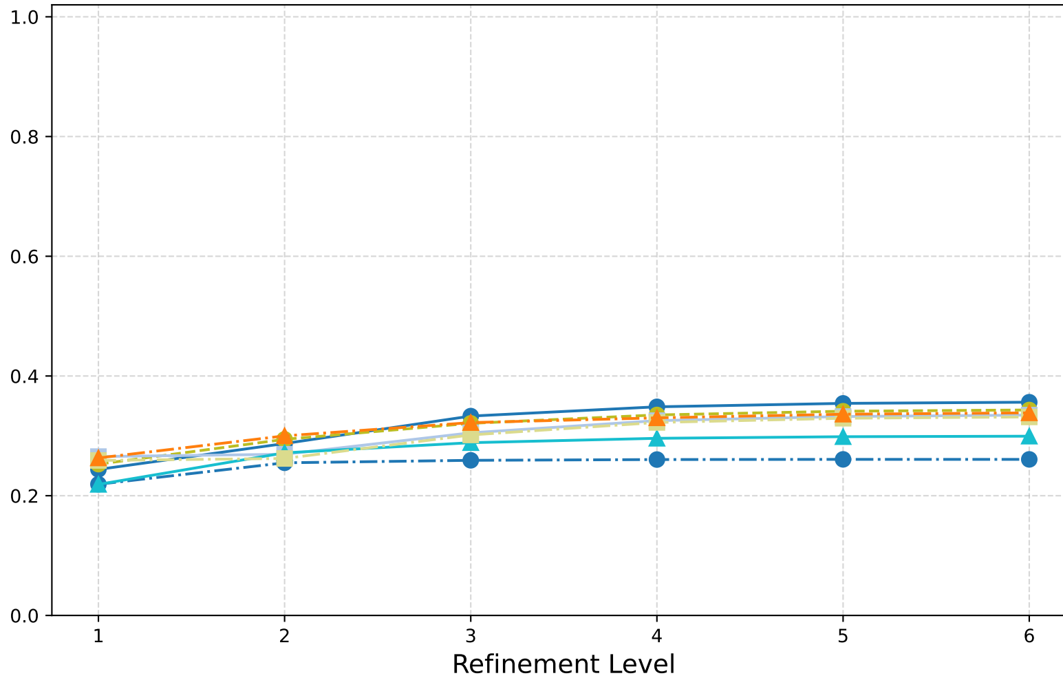
Dirac: W-Cycle (Row Sum) - Spectral Radii
