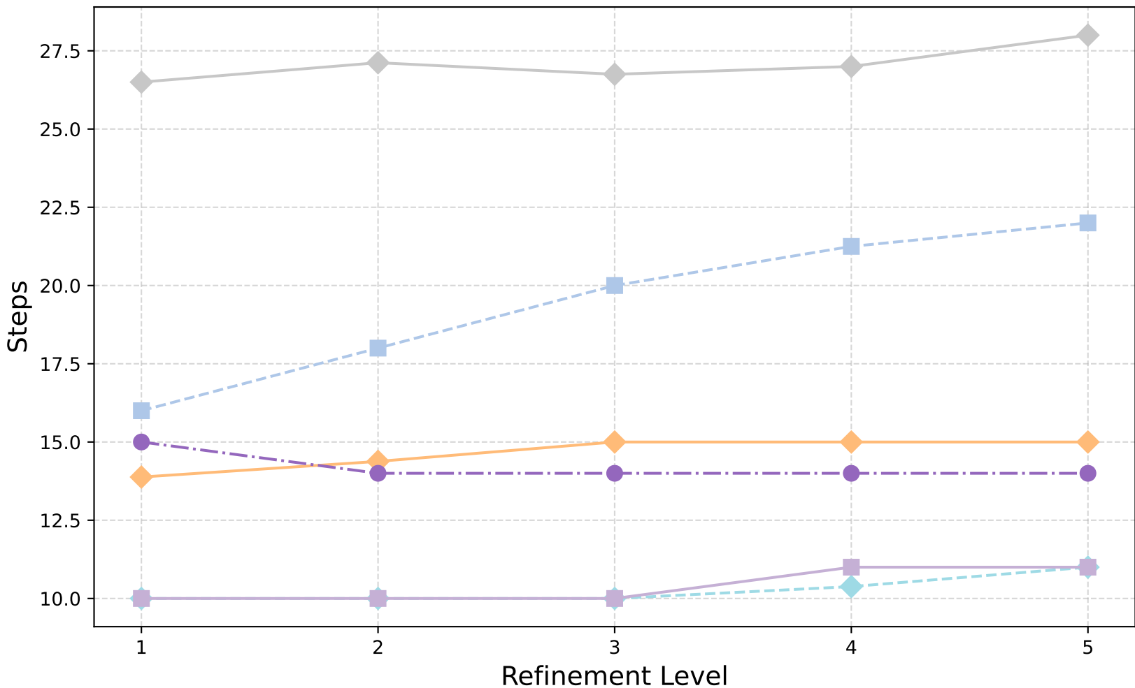
Dirac: W-Cycle (Row Sum) - GMRES Iterations
