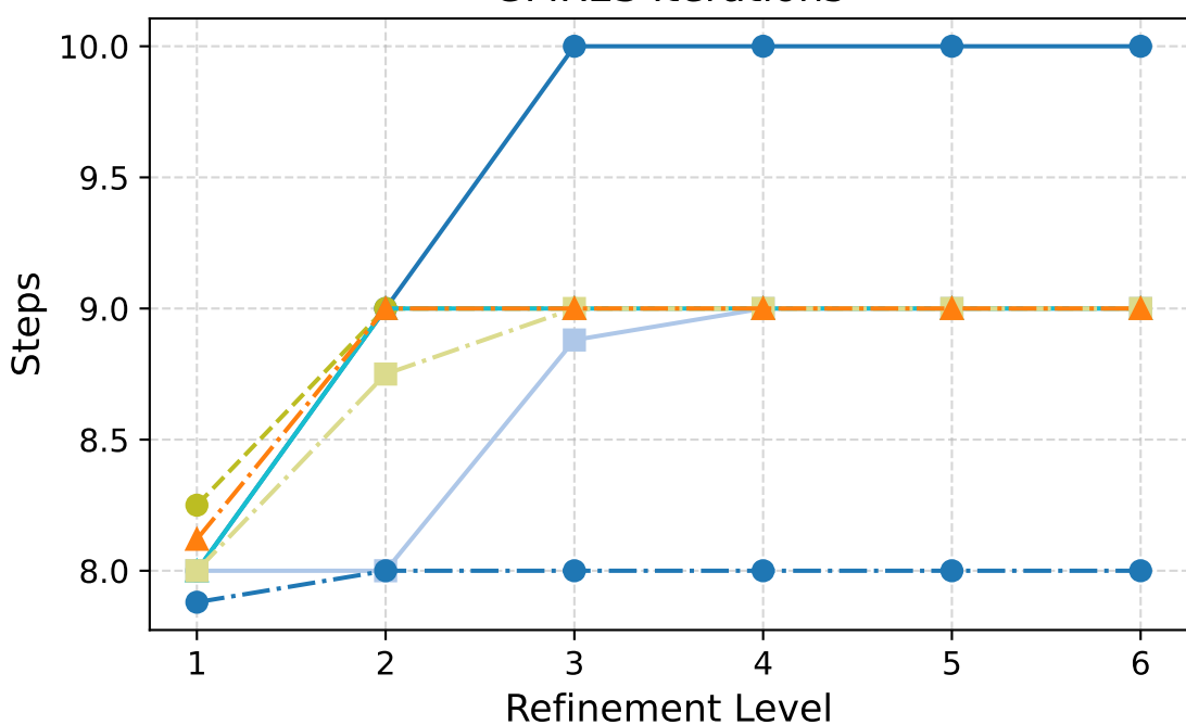
GMRES Iterations
