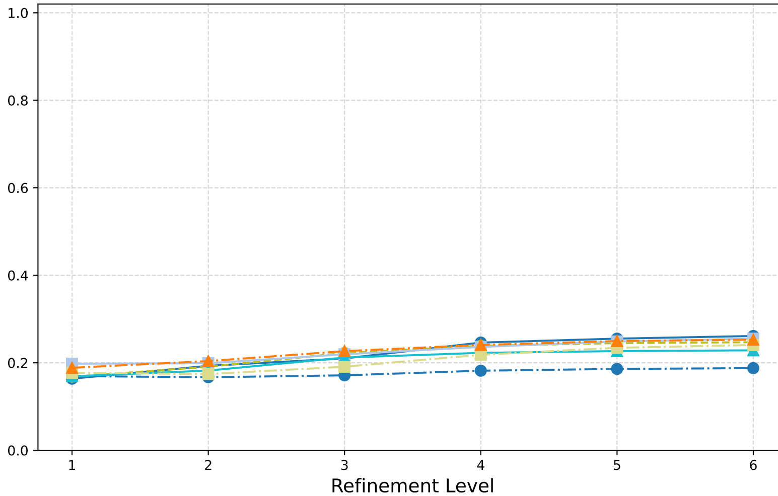
1-form Hodge Laplacian: W-Cycle (Row Sum) - Spectral Radii
