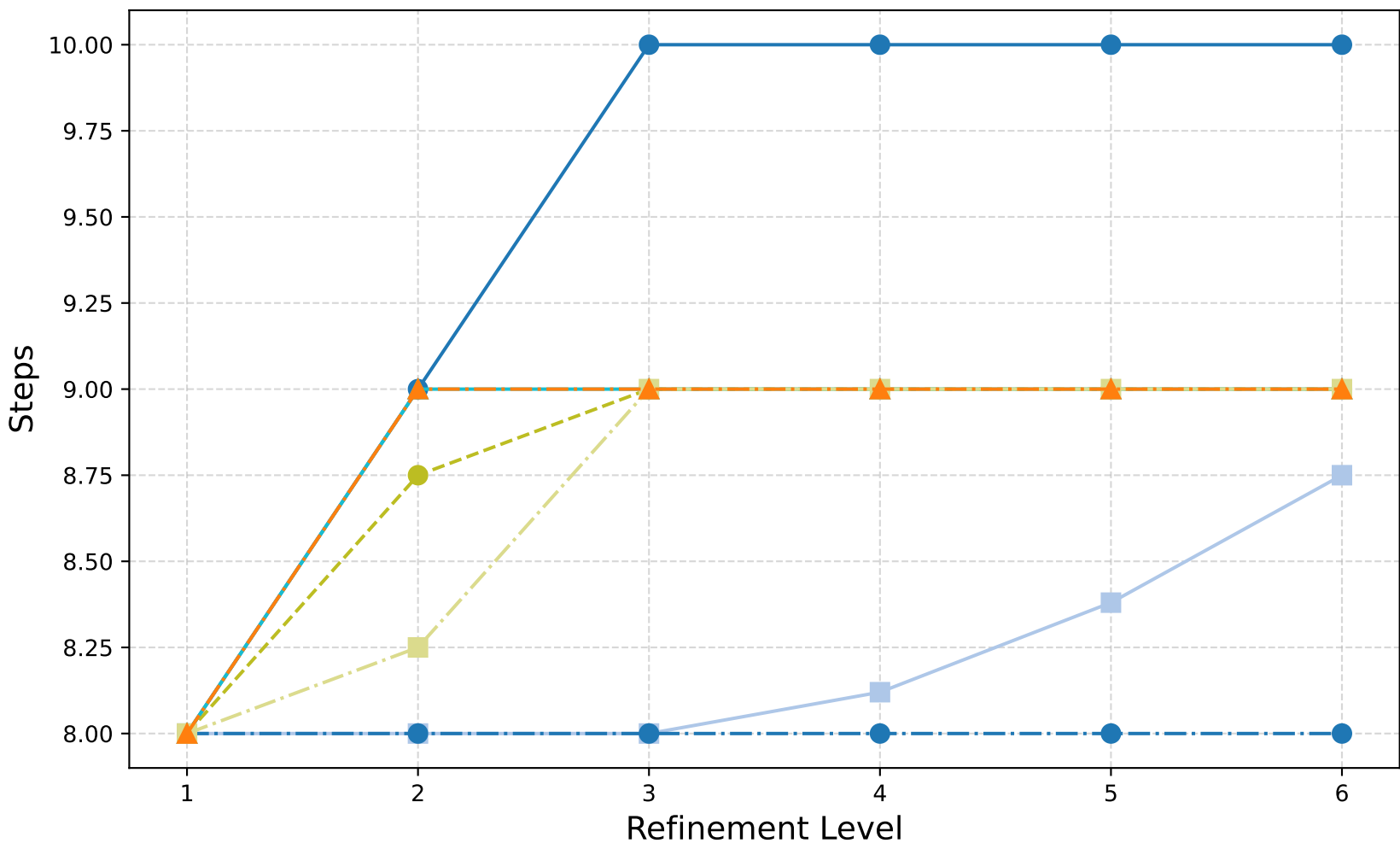
1-form Hodge Laplacian: W-Cycle (Row Sum) - GMRES Iterations
