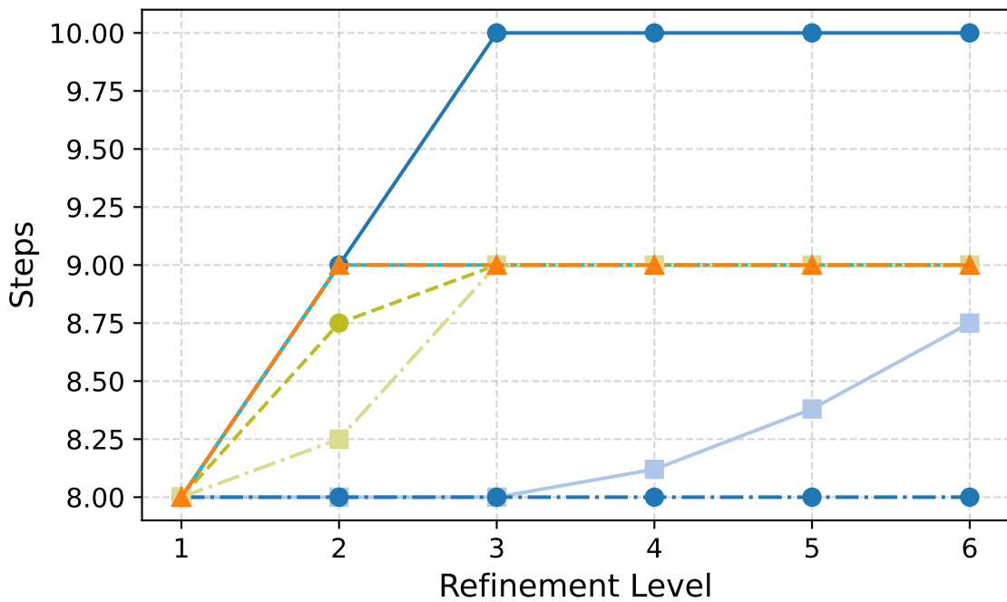
GMRES Iterations
