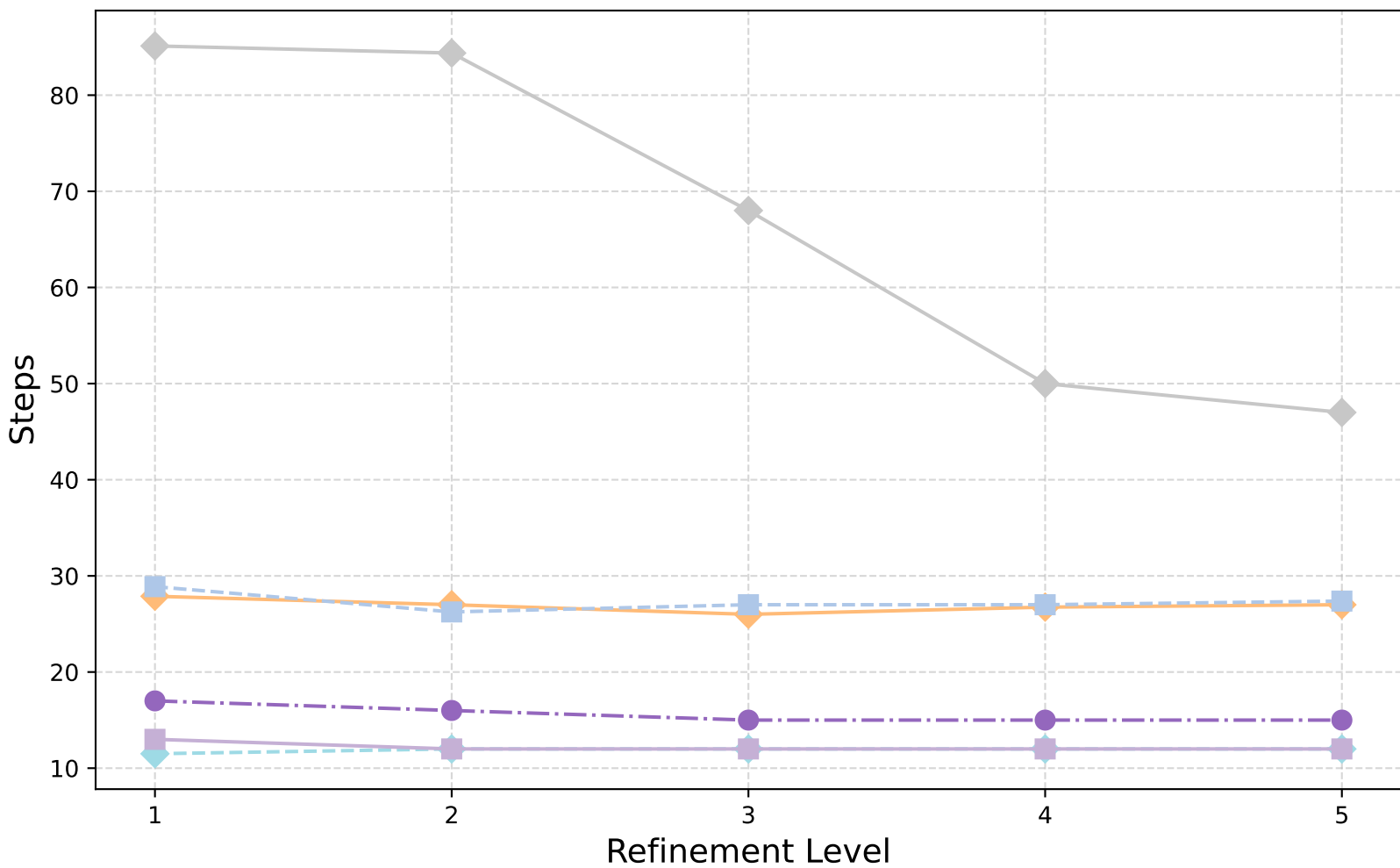
Dirac: V-Cycle (Scaled Id) - GMRES Iterations
