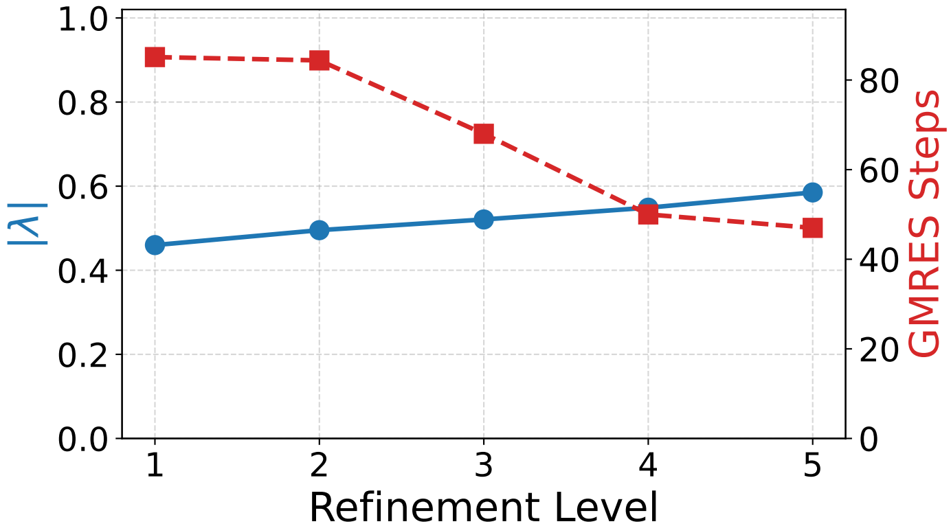
Dirac: V-Cycle (Scaled Id)
